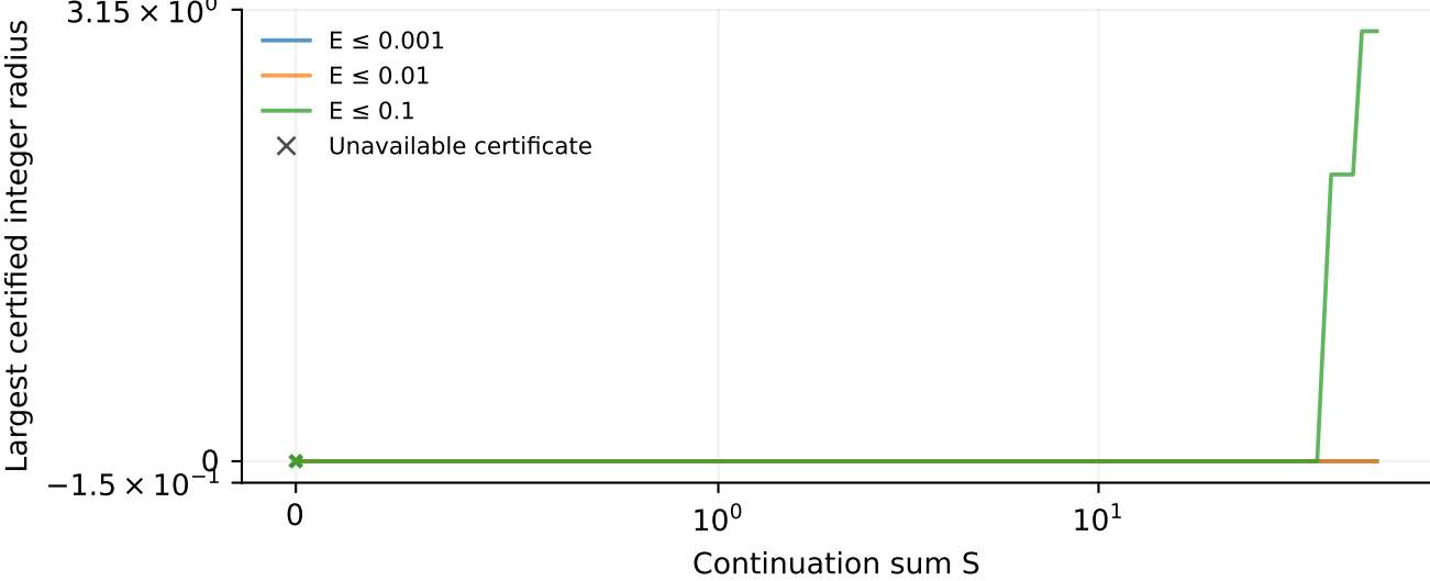
Certified radius from uniform bound; no evaluation-lag cap
