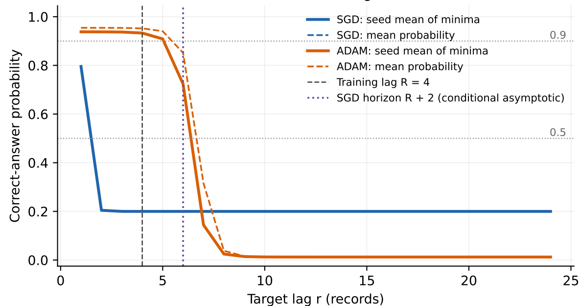
Learned retrieval gate
