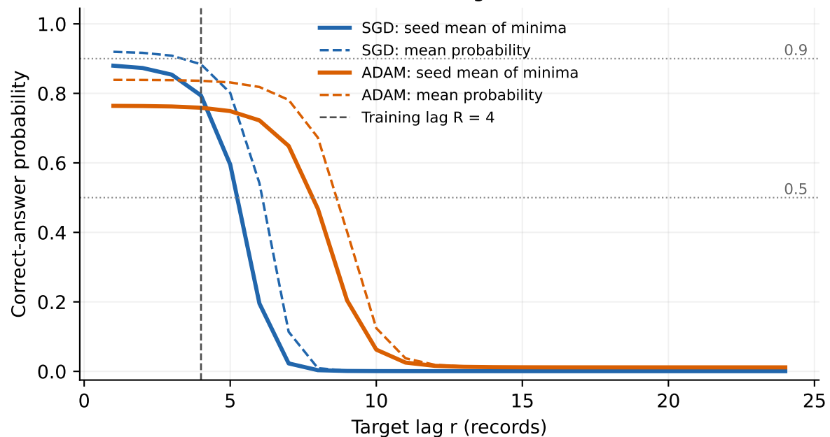
Frozen retrieval gate (ALiBi)
