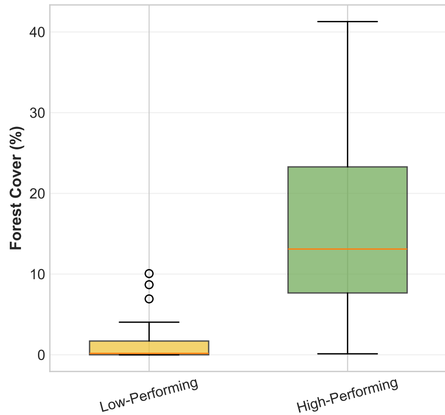
Forest Cover
