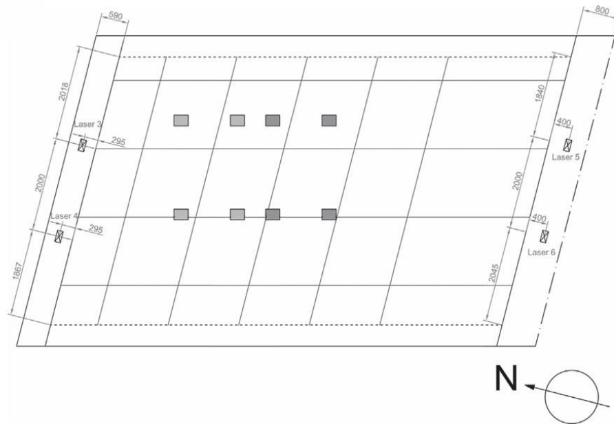
Figure 4.8 – Instrumentation layout on the bottom of the slab [1].
