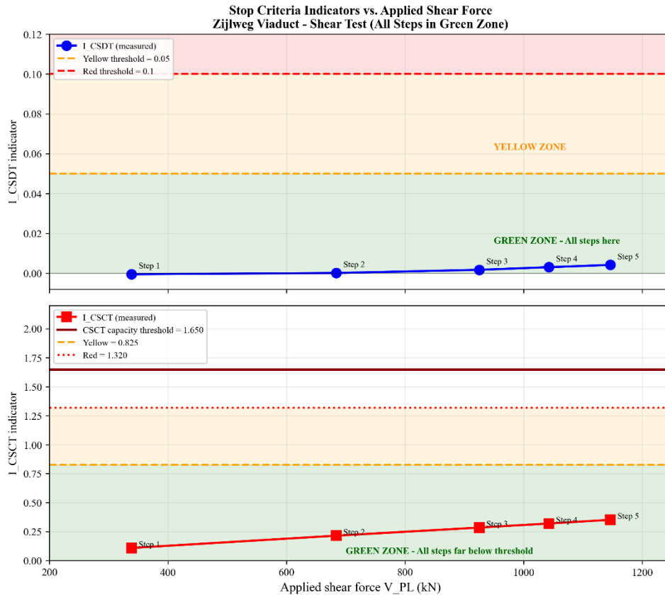
Figure 5.6 – Stop criteria indicators throughout the shear proof load test, all remaining in the green light zone.
