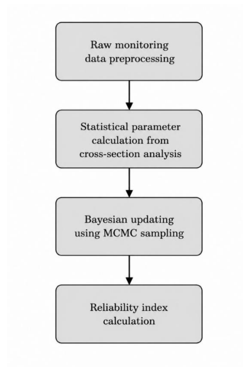
Figure 3.2 – The Complete analysis workflow
