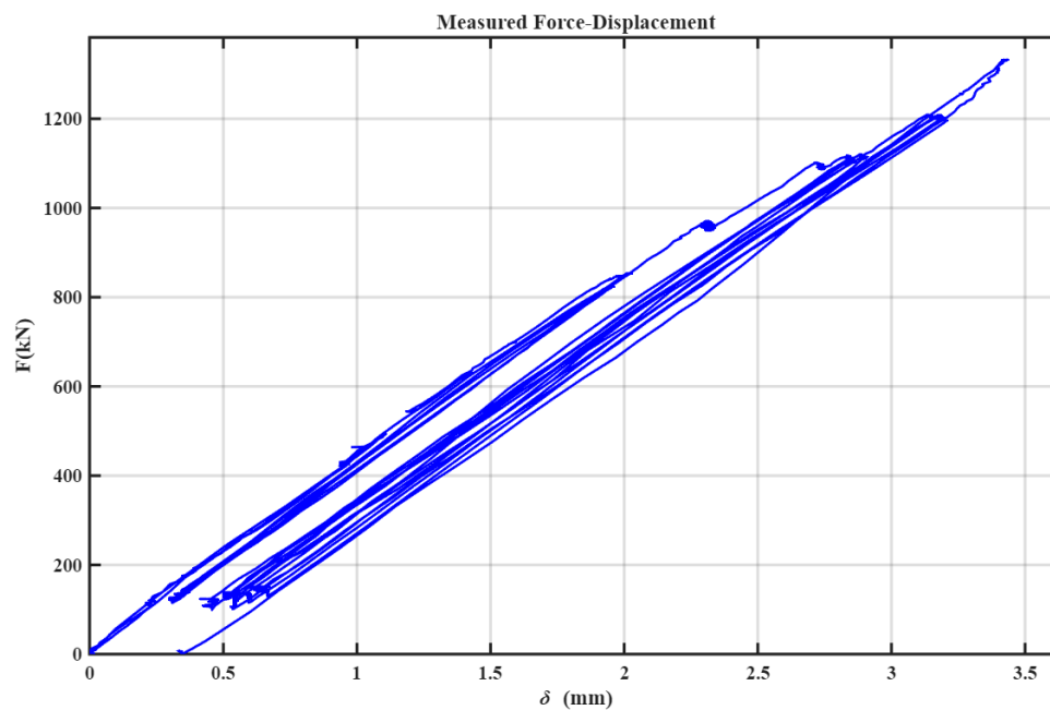
Figure 4.10 – Load-displacement envelope for bending moment proof load test.
