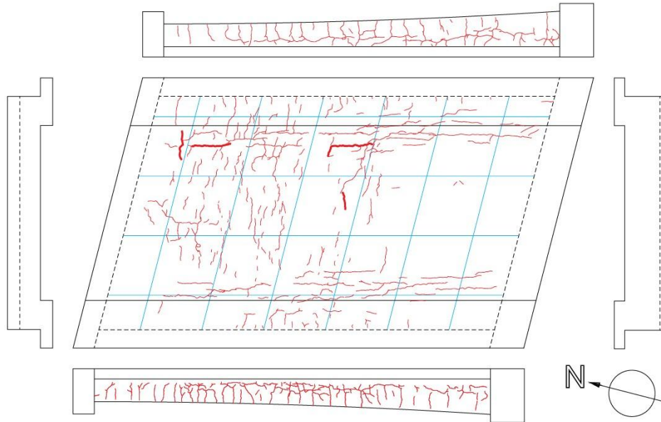
Figure 4.9 – Location of monitored cracks during the proof load tests [1].
