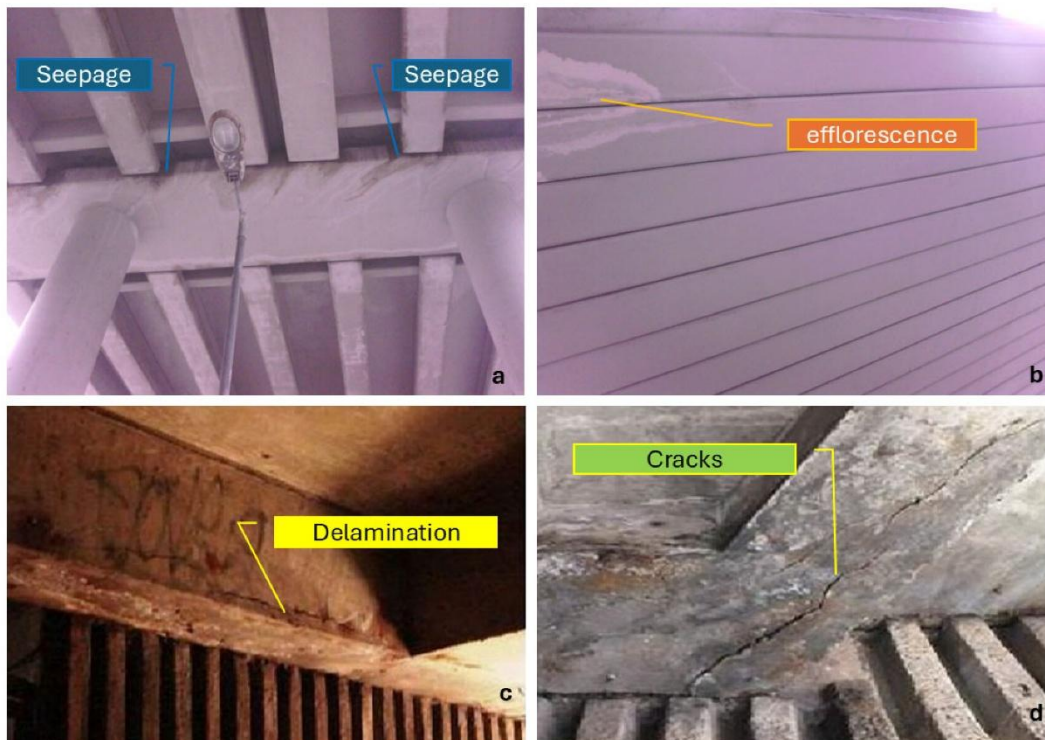
Figure 1.2 – Common deterioration mechanisms in aging concrete bridges.
