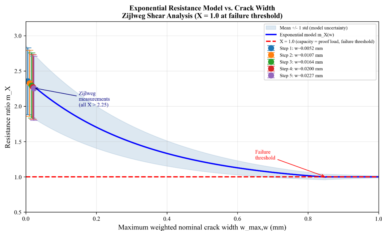
Figure 5.4 – Exponential resistance model showing how X approaches 1.0 at failure. The five Zijlweg crack width measurements correspond to the high- X region, confirming absence of shear damage.
