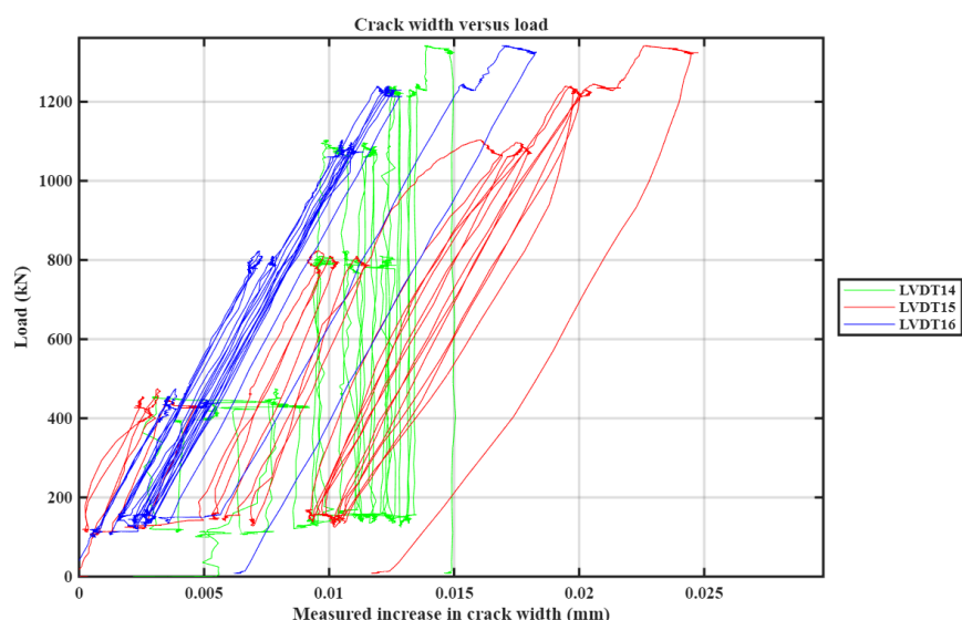
Figure 4.13 – Crack width measurements vs. applied load for shear test.
