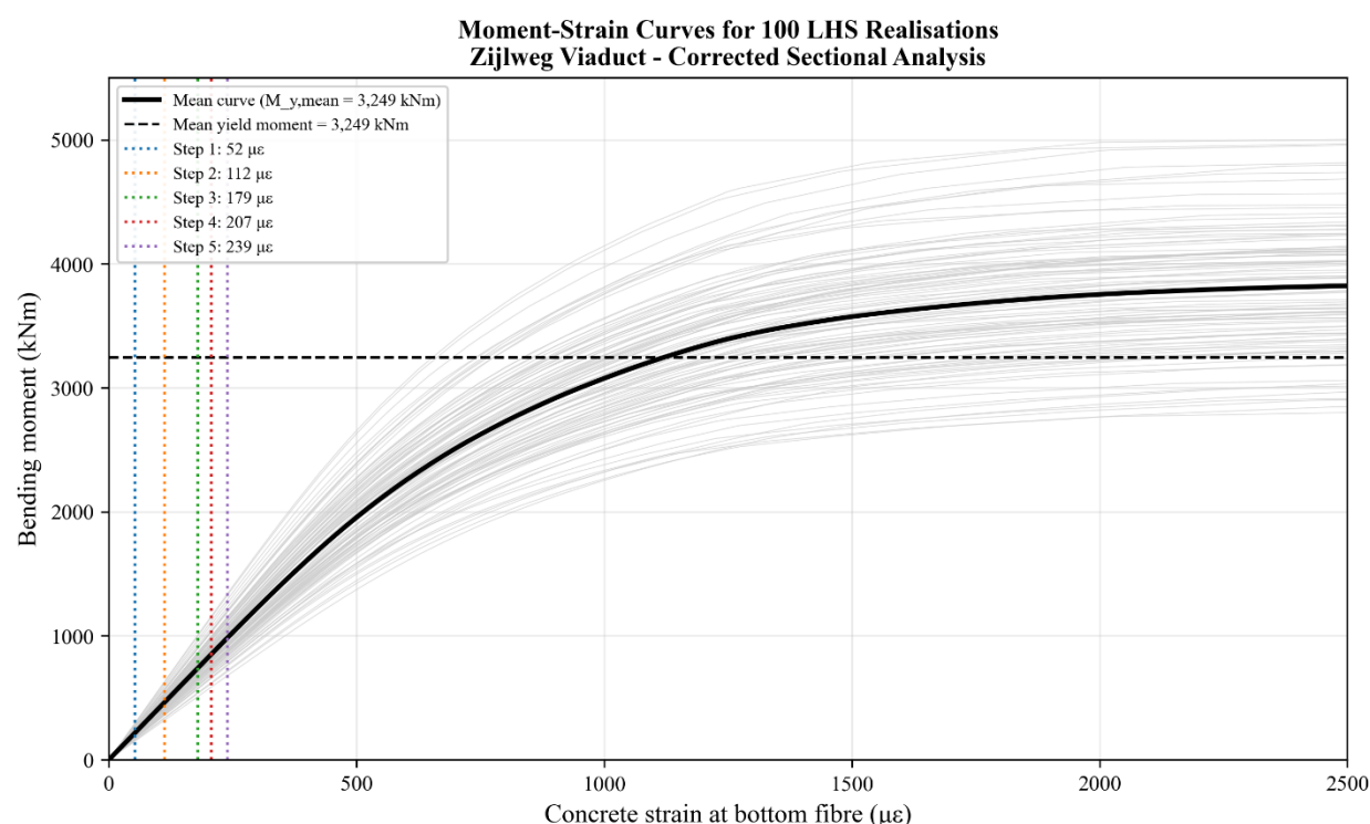
Figure 5.1 – Moment-strain curves for 100 LHS realisations showing the Zijlweg cross-section capacity.
