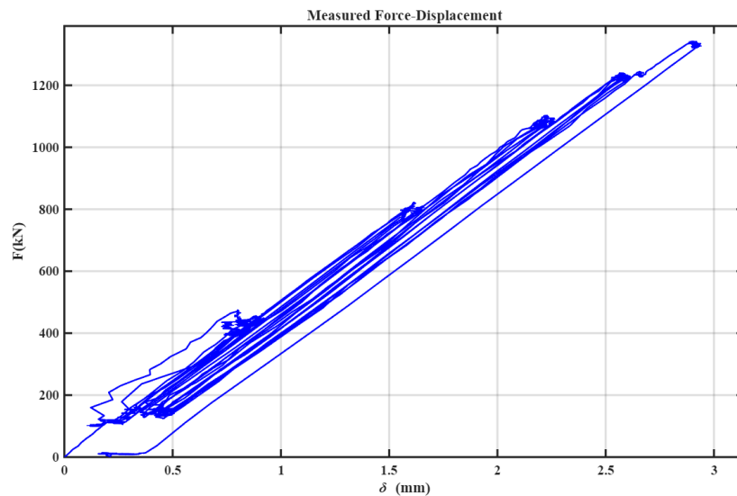
Figure 4.12 – Load-displacement envelope for shear proof load test.
