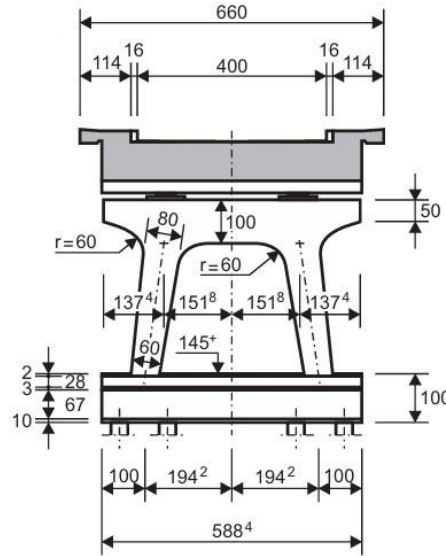
Figure 4.2 – Cross-section of viaduct Zijlweg [1].
