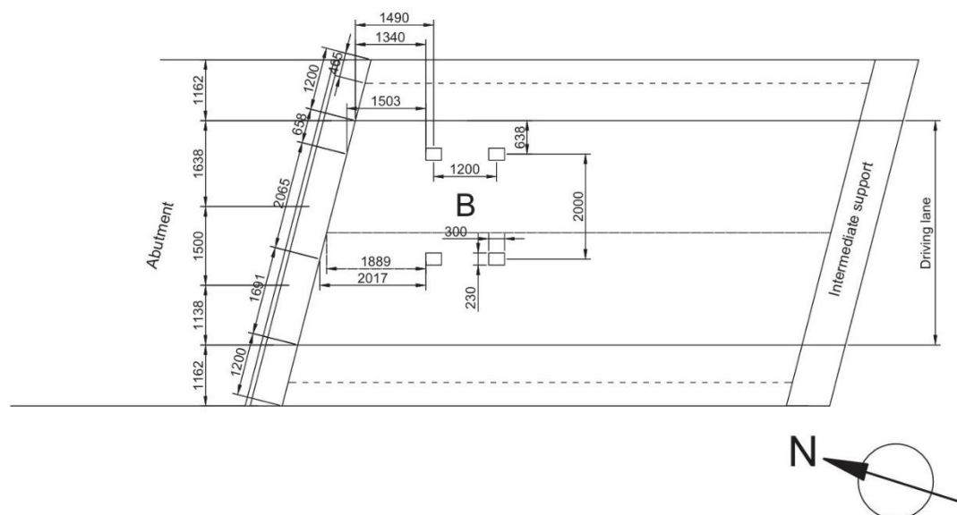
Figure 4.6 – Load positions for bending and shear proof load tests [1].
