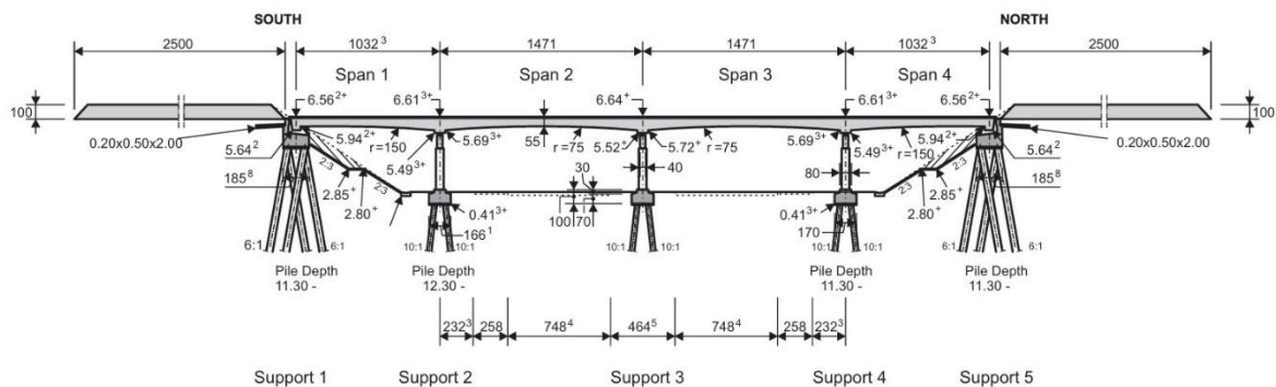
Figure 4.1 – Longitudinal section of viaduct Zijlweg [1].
