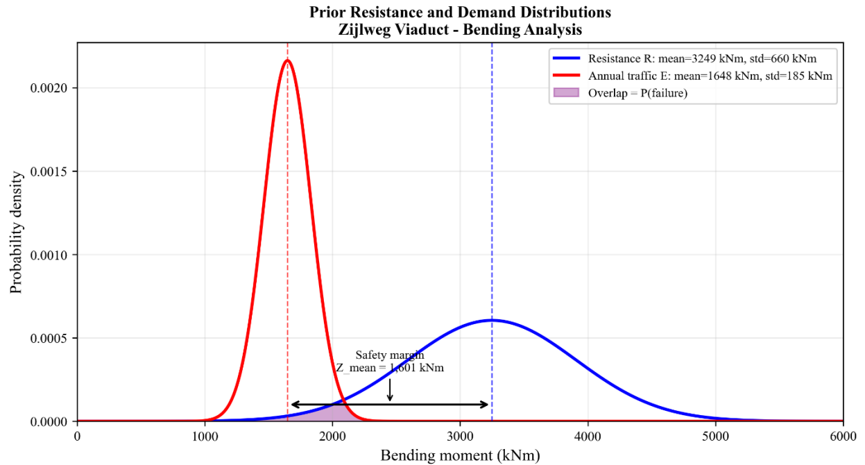
Figure 5.2 – Prior resistance and demand distributions for the Zijlweg bending analysis showing the safety margin of 1,601 kNm at mean values.
