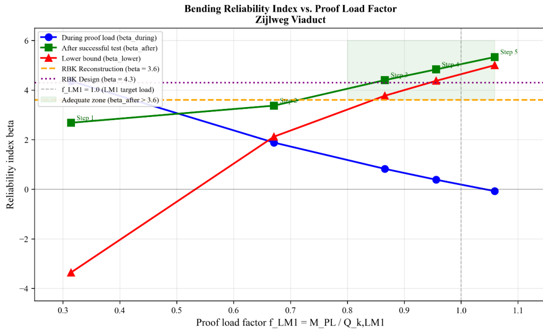
Figure 5.3 – Bending reliability index vs. proof load factor showing the Bayesian update increasing \beta_{\text{after}} from 2.68 to 5.33 across the five load steps.
