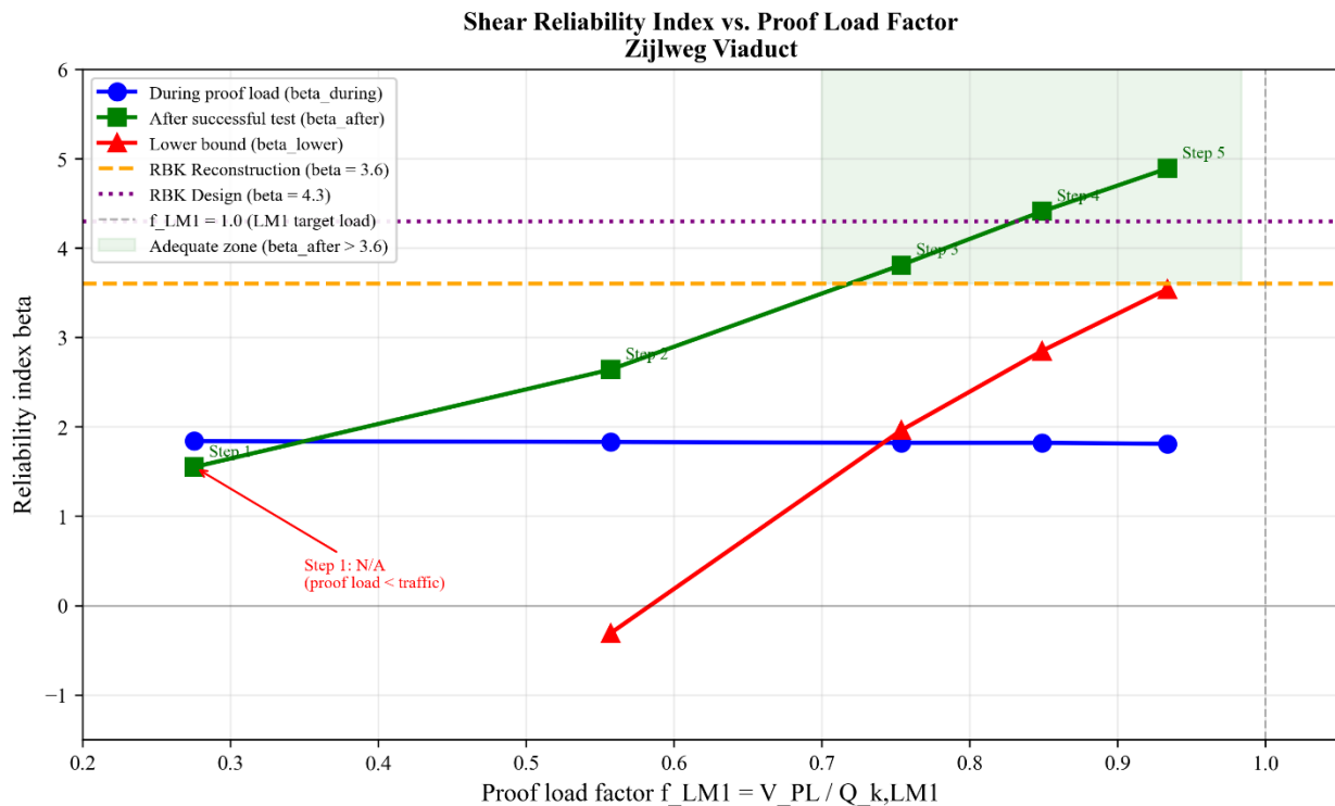
Figure 5.5 – Shear reliability index vs. proof load factor showing \beta_{\text{after}} increasing from 1.55 to 4.89 across the five load steps.
