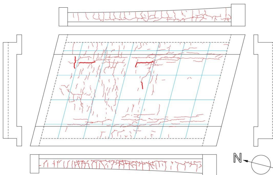
Figure 4.4 – Pre-existing crack pattern in span 4 of viaduct Zijlweg [1].
