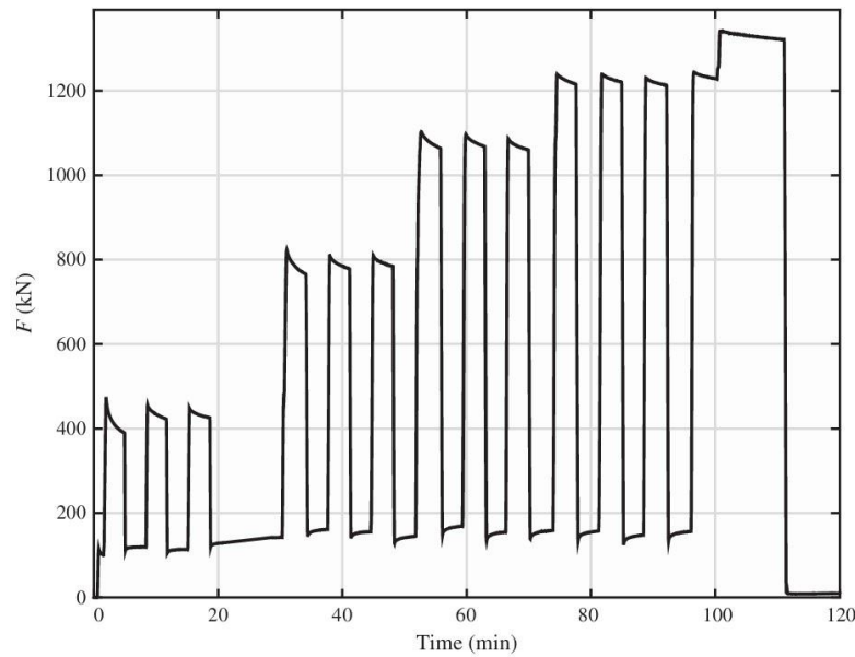
Figure 4.7 – Loading protocol for bending and shear proof load tests [1].
