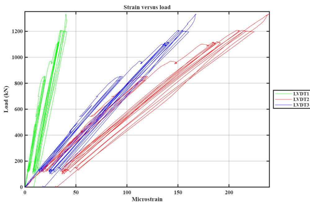
Figure 4.11 – Measured concrete strains vs. applied load for bending test.
