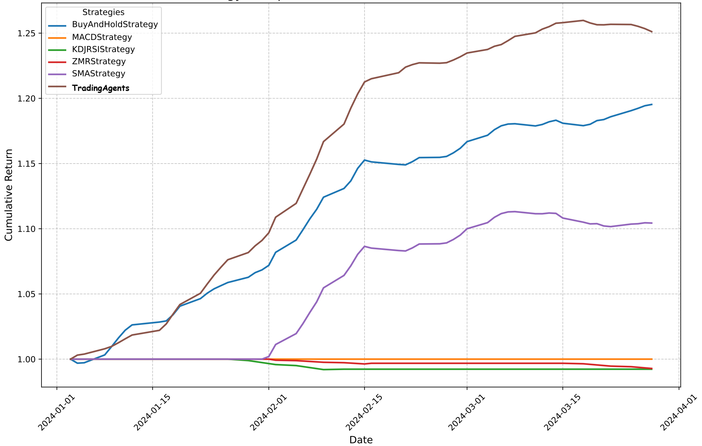
Strategy Comparison - Cumulative Returns for AMZN
