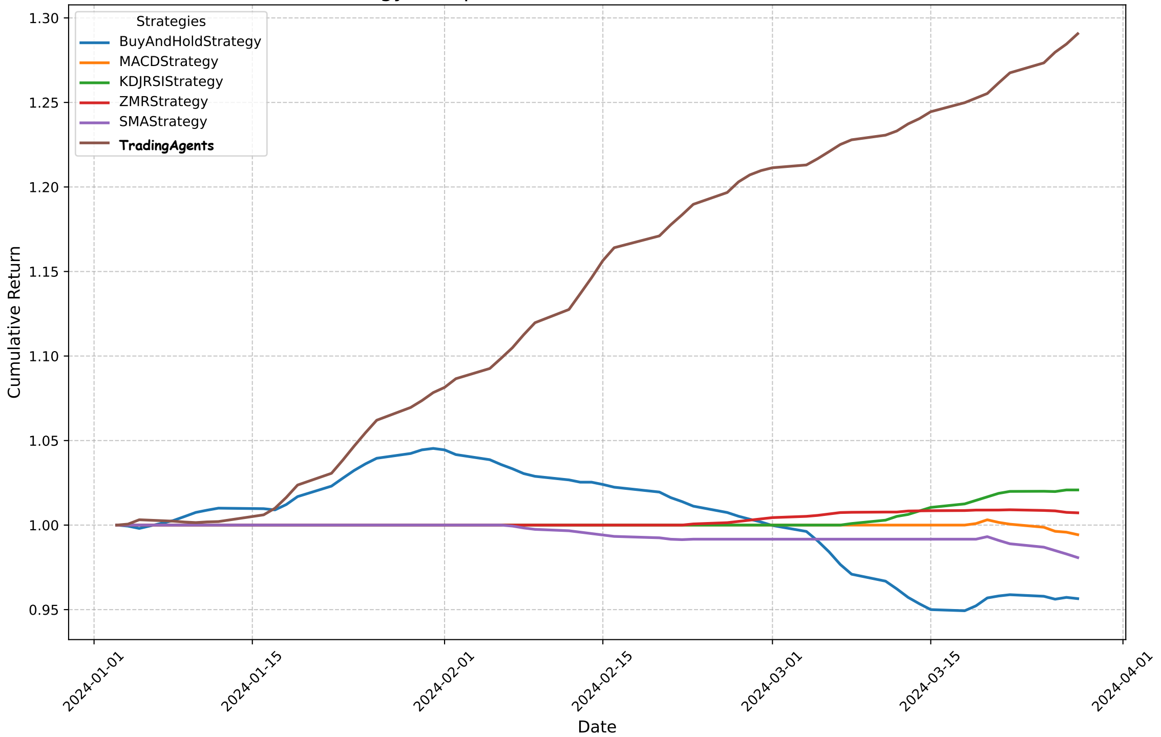
Strategy Comparison - Cumulative Returns for AAPL
