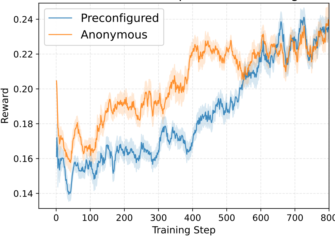
Duo-MARFT (Non-parameter-sharing)
