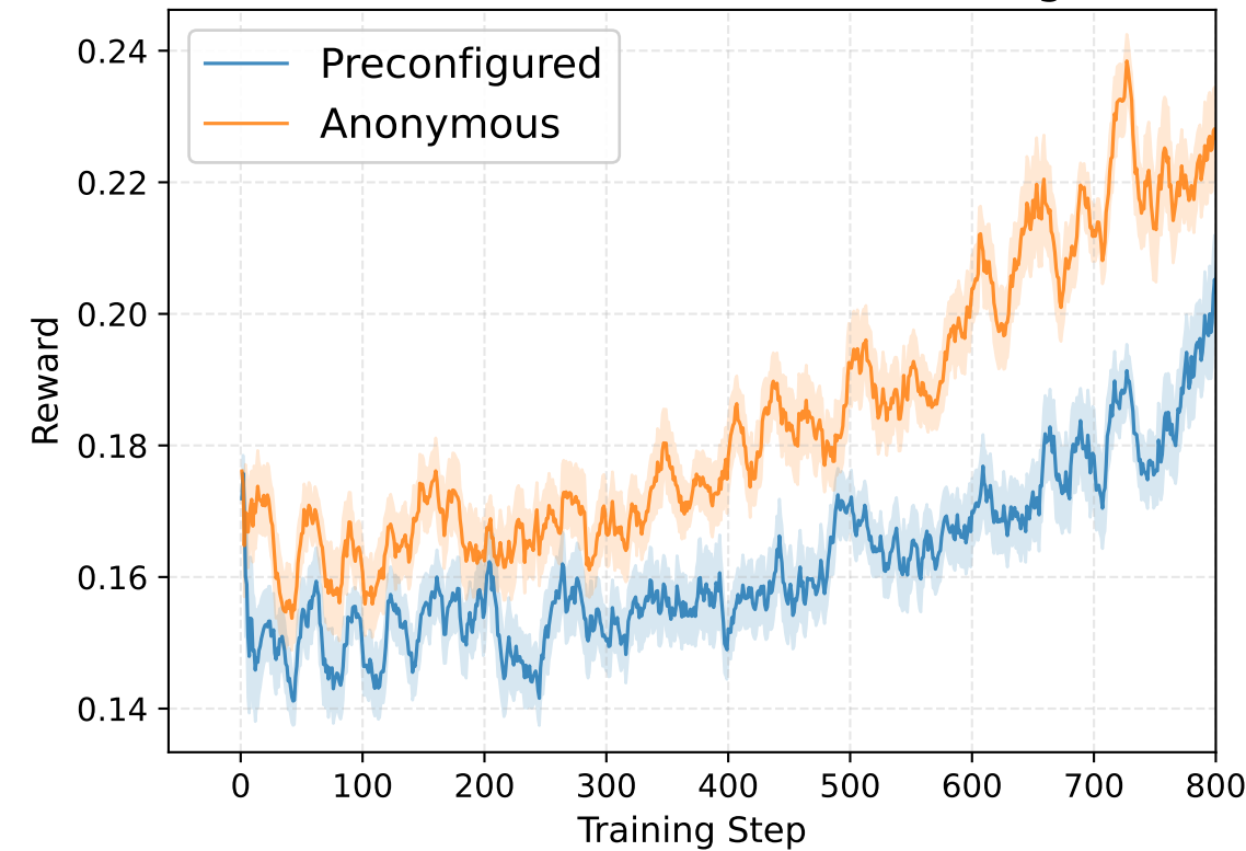
Quad-MARFT (Non-parameter-sharing)
