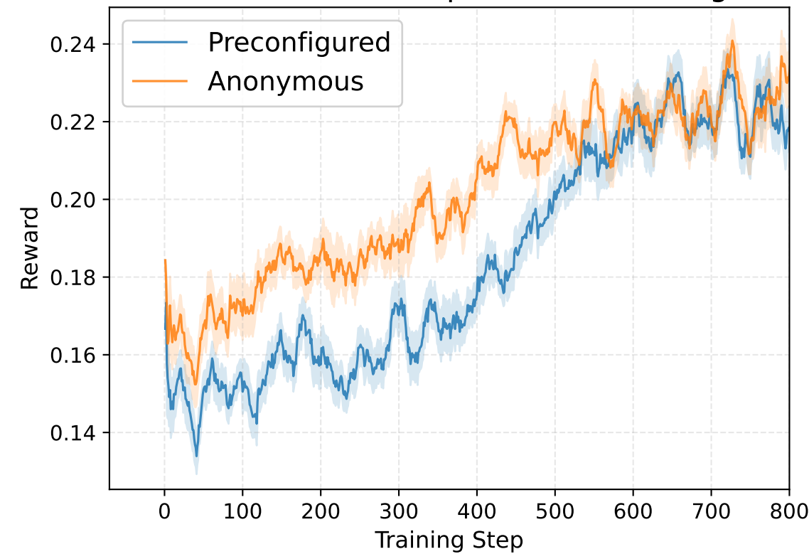
Quad-MARFT (Non-parameter-sharing)
