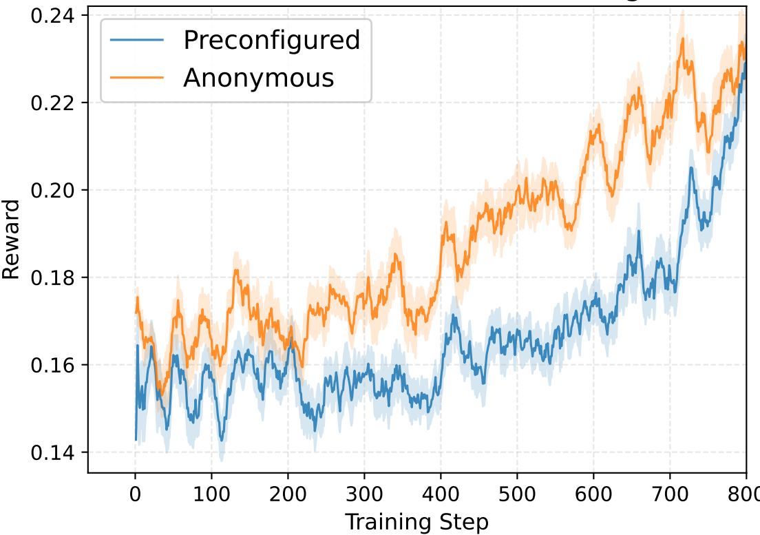
Duo-MARFT (Non-parameter-sharing)
