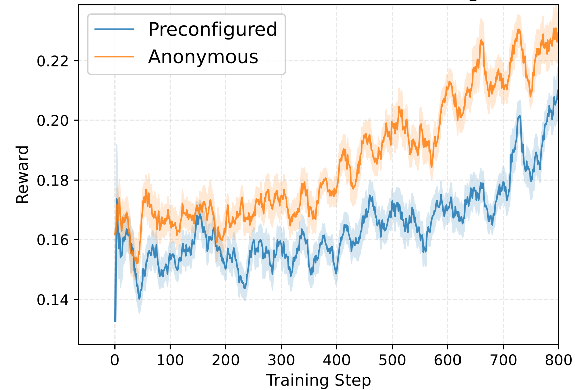
Trio-MARFT (Non-parameter-sharing)
