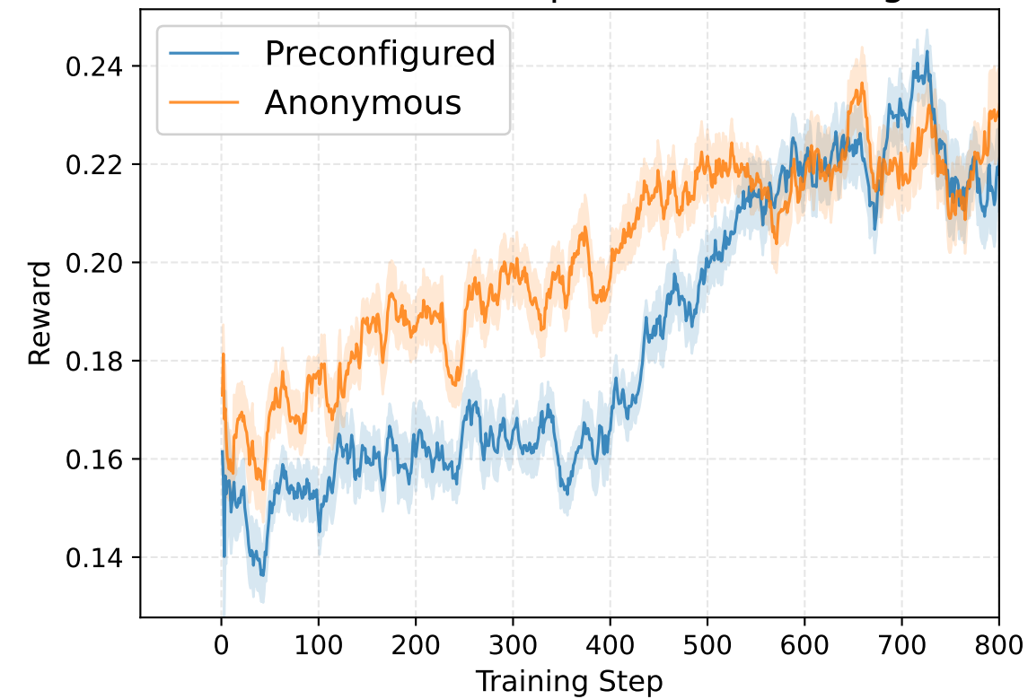
Trio-MARFT (Non-parameter-sharing)
