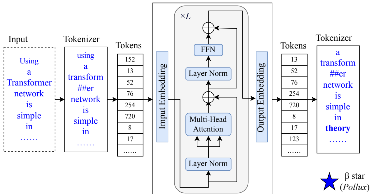
(a) LLM - "Next-token prediction"
