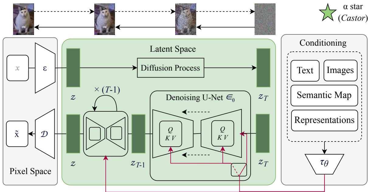
(b) Stable Diffusion - "Denoising by noise estimation at each time step"
