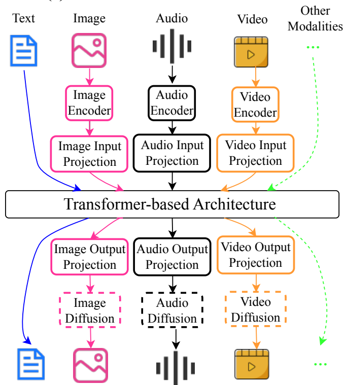
(c) Multimodal Generative Model
