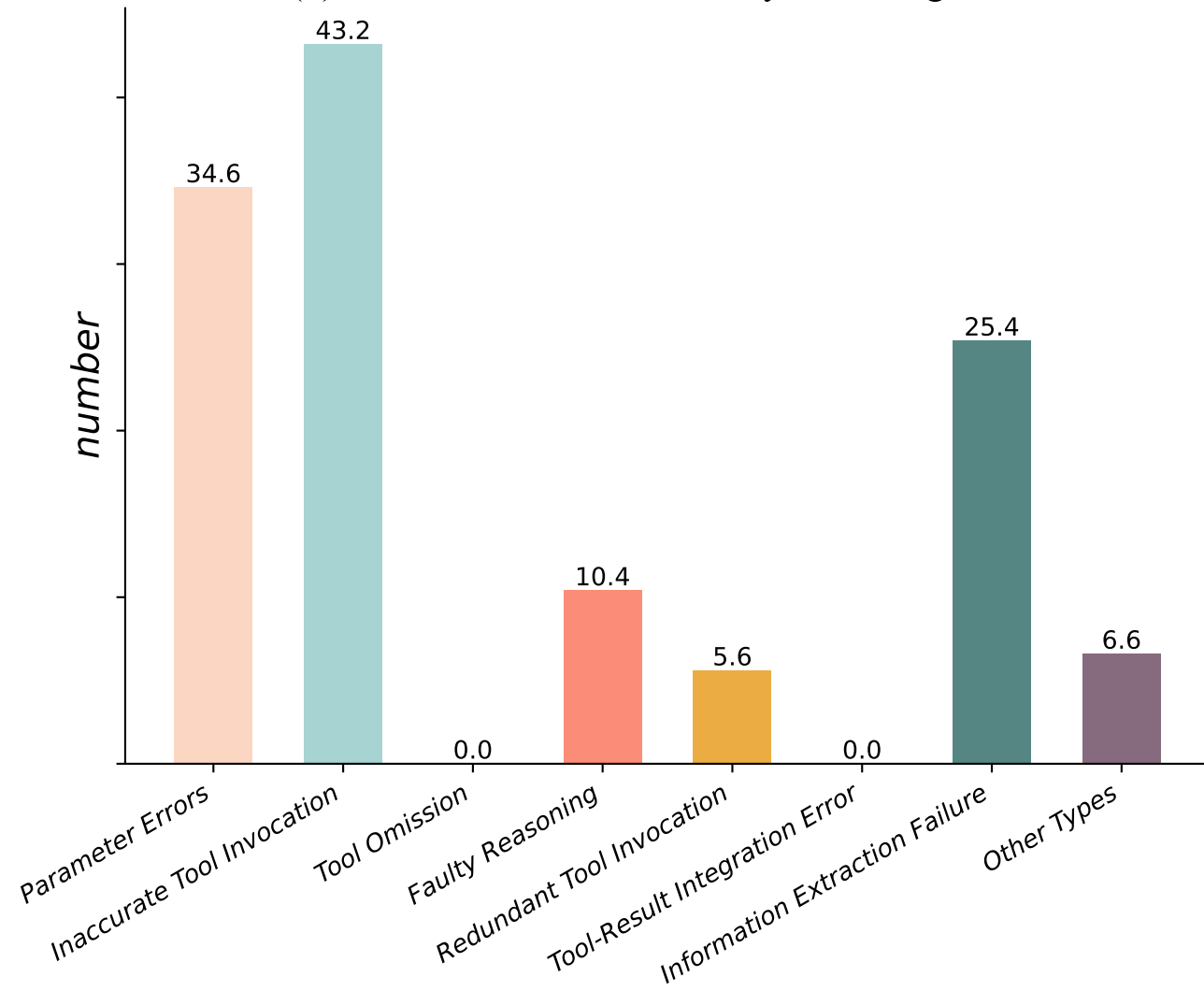
(b) Error Distribution of Fuzzy Matching Tasks
