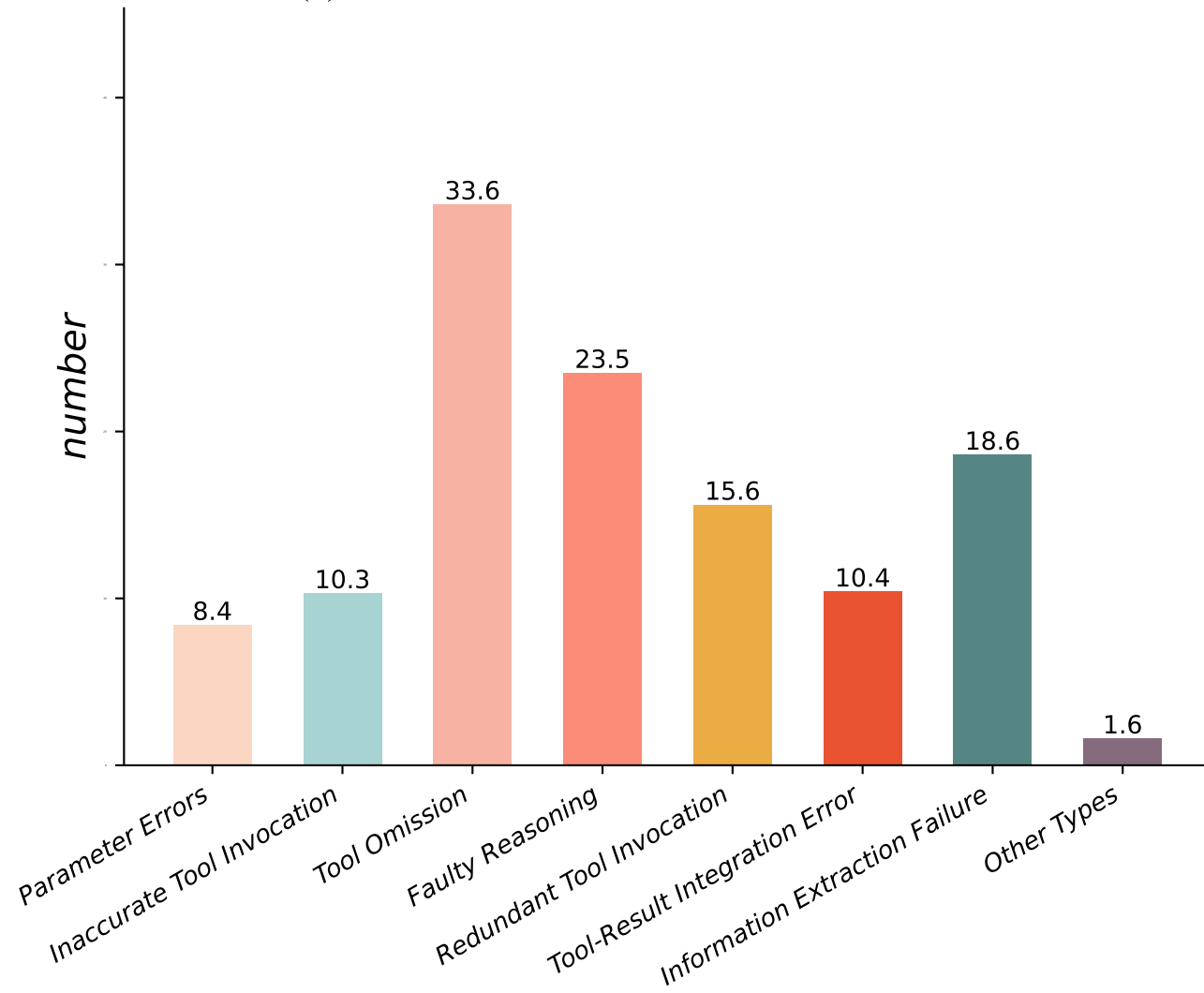
(a) Error Distribution of Precise Answer Tasks
