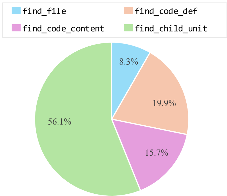
(a) Search-tool invocation distribution of Issue Localization Agent
