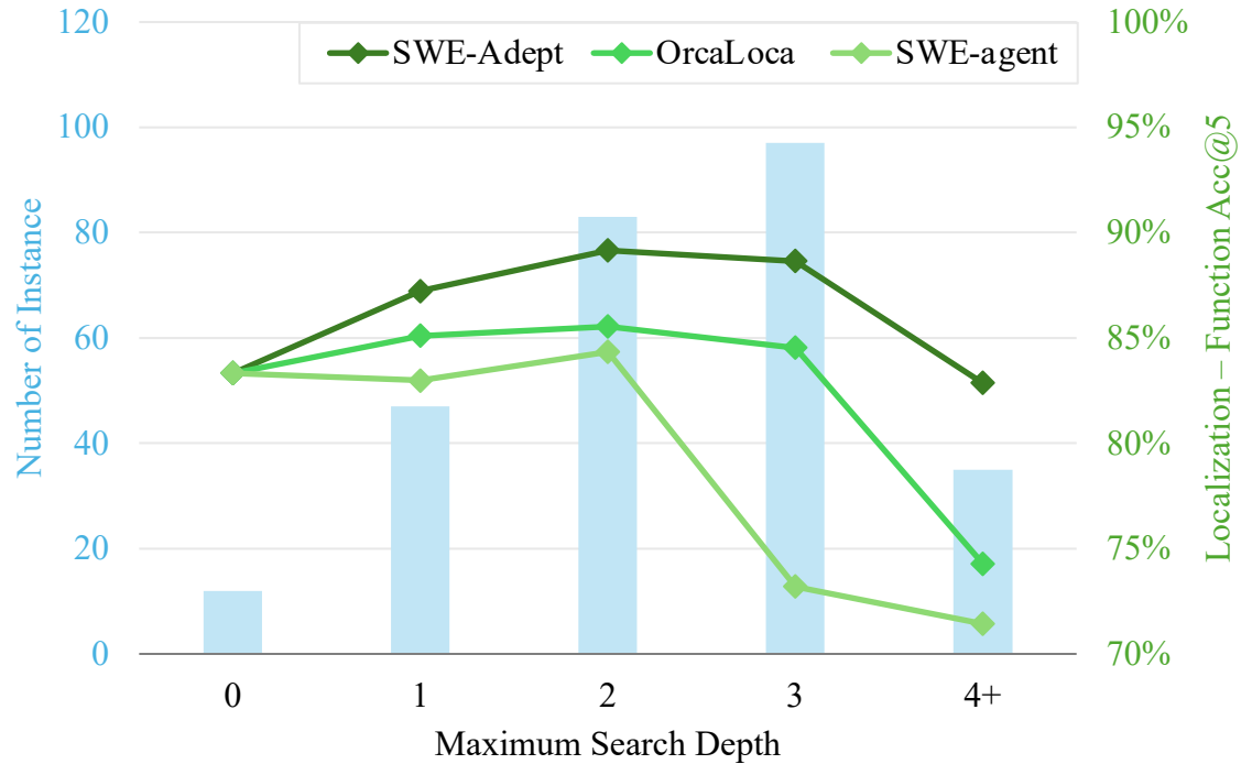
(b) Instance distribution and localization accuracy by maximum search depth
