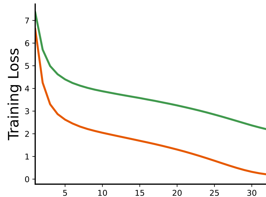
CC12M
