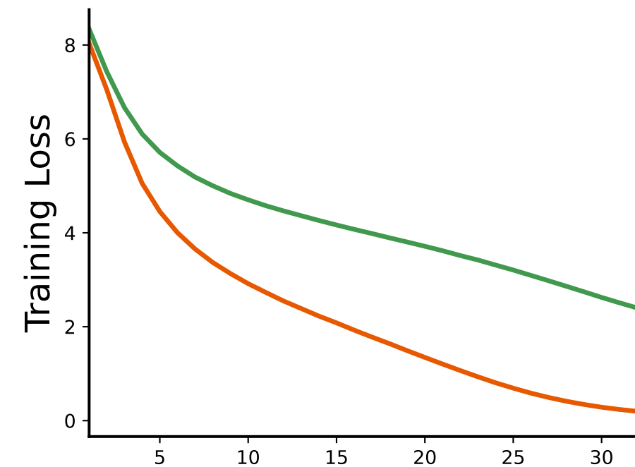
CC3M
