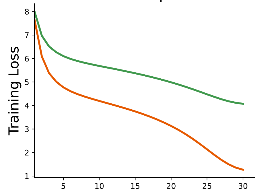
Redcaps
