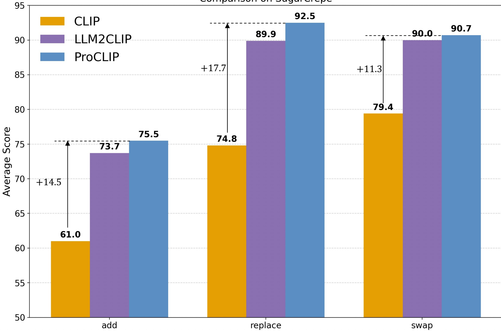
Comparison on SugarCrep
