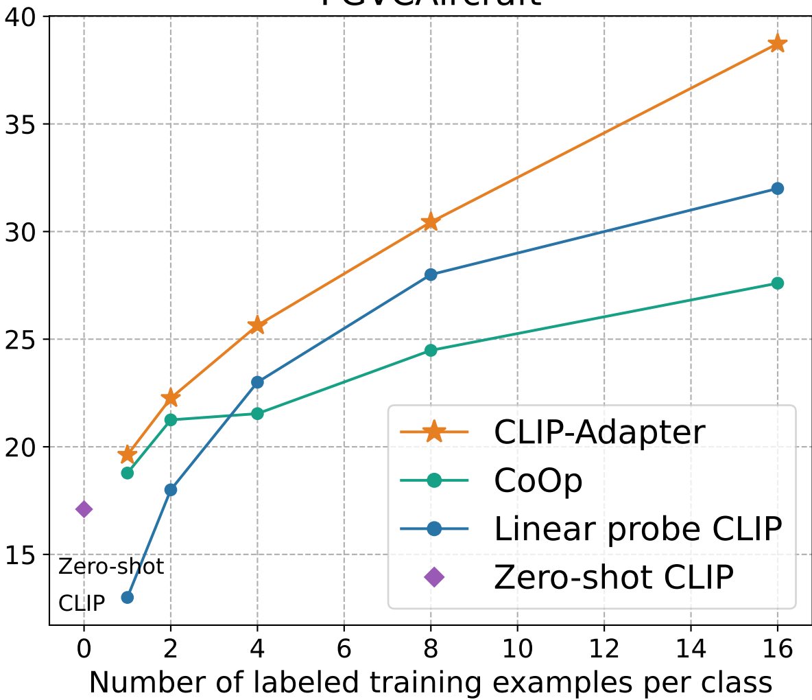
FGVCAircraft
