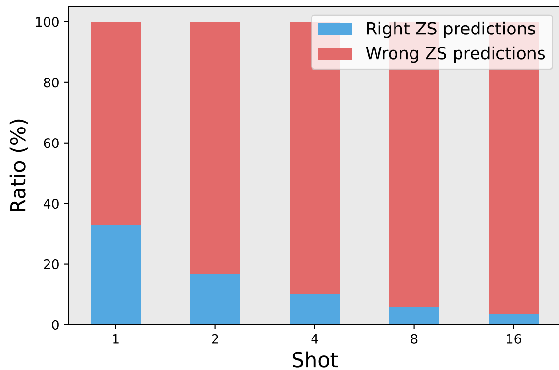
(b) Failure cases analysis on Oxford Flowers
