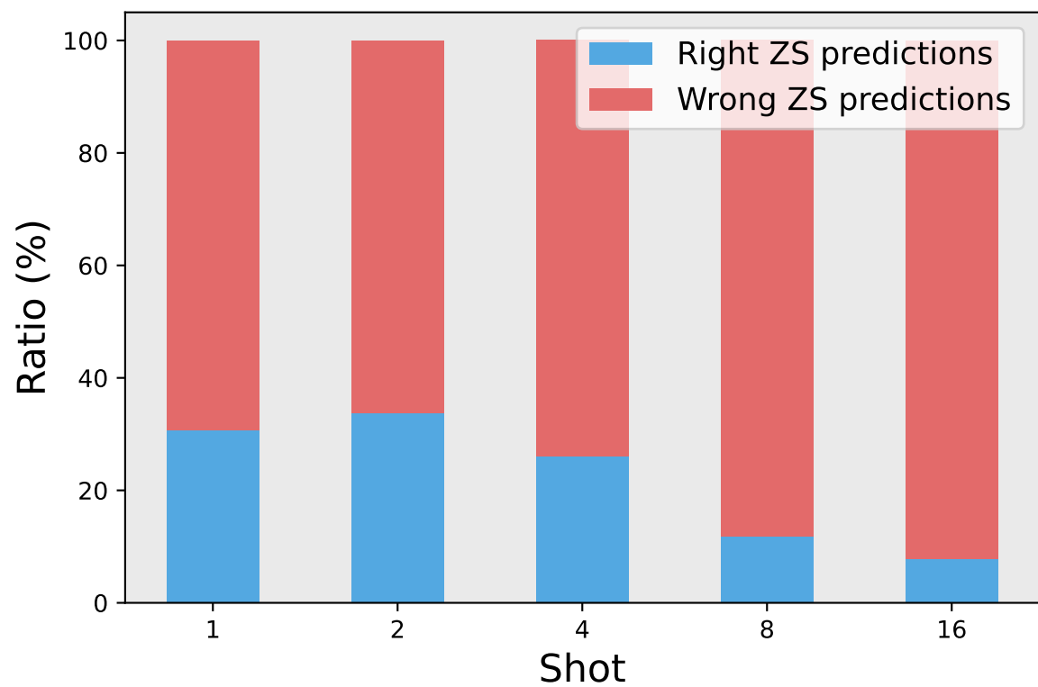
(a) Failure cases analysis on EuroSAT
