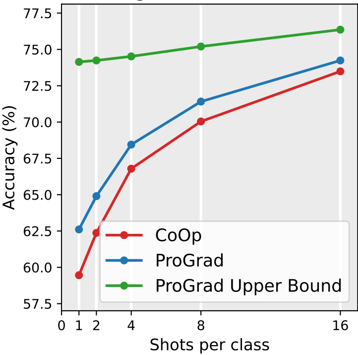
Average over 11 datasets
