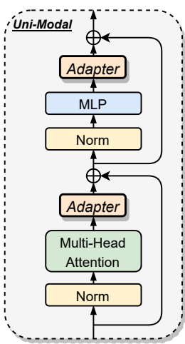
Vision/Language Encoder Layer
