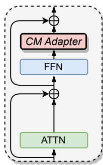
Sequential ffn
