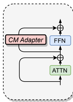
Parallel ffn
