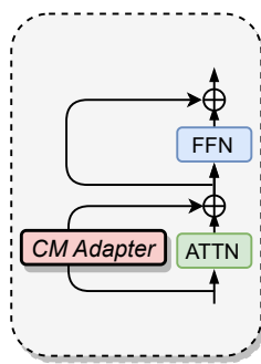
Parallel attn
