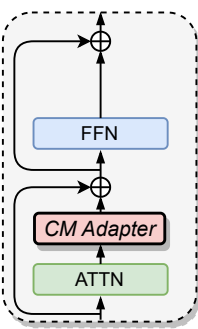
Sequential attn
