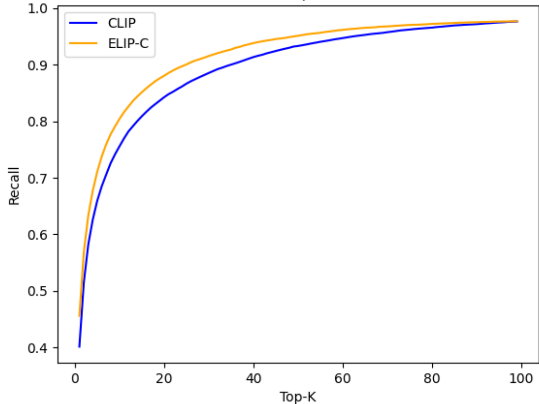
Recall - TopK Curve
