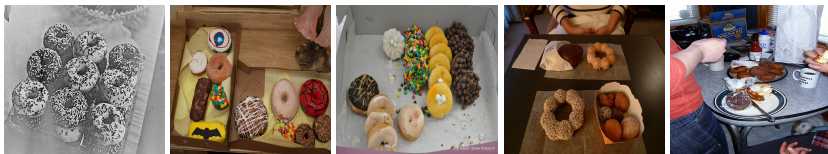
Initial Ranking
