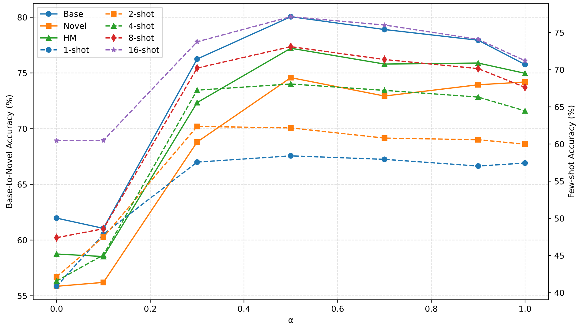
Effect of Fusion Coefficient \alpha on Both Base-to-Novel and Few-shot Performance
