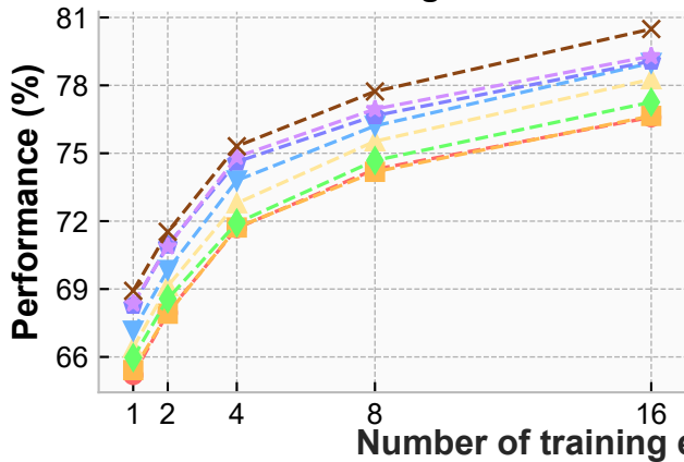
Average
