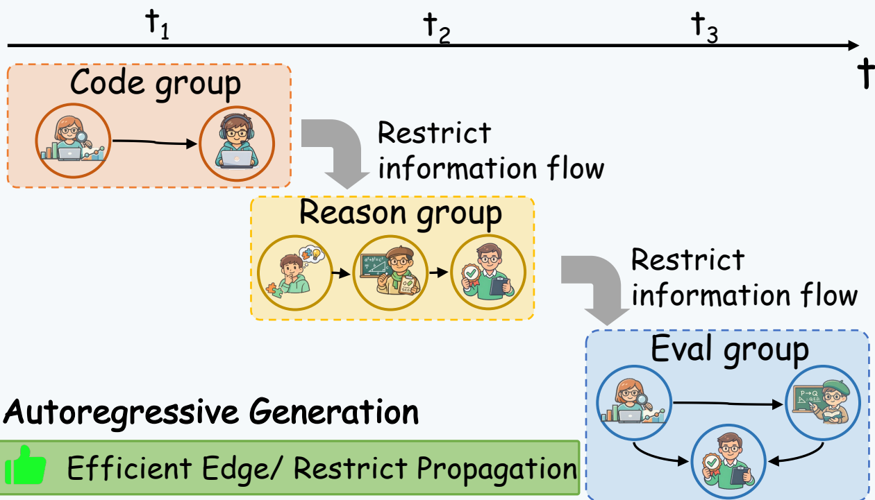
(b) Group-centric Paradigm (Ours)
