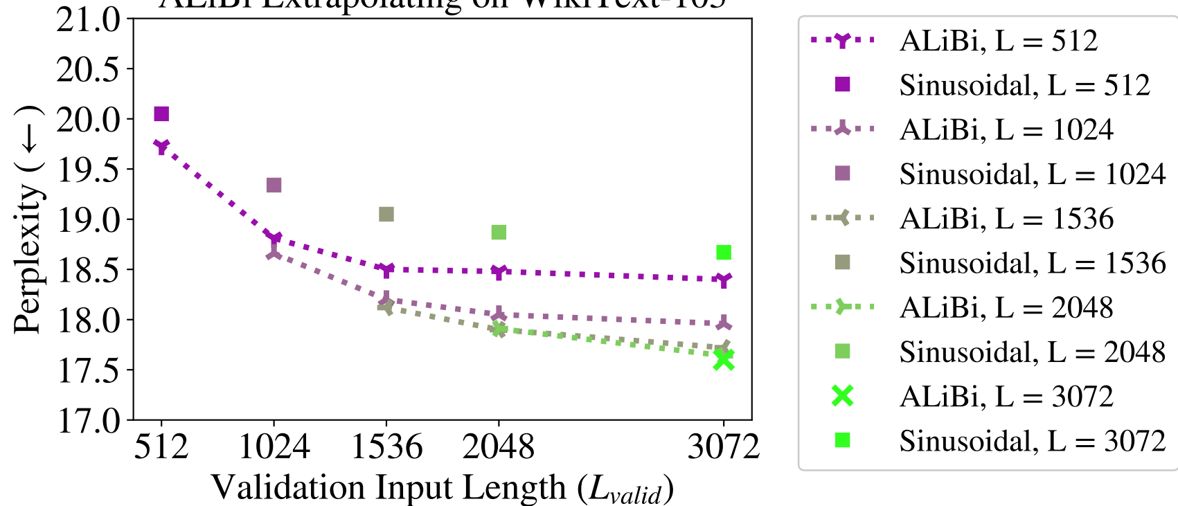
ALiBi Extrapolating on WikiText-103
