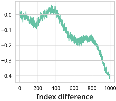
Head 16
