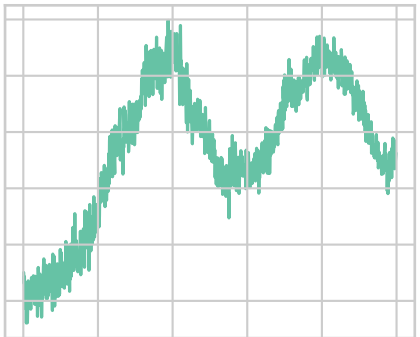
Head 20
