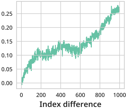
Head 32
