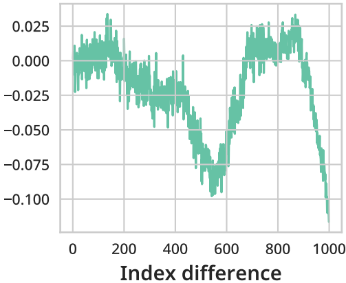
Head 8
