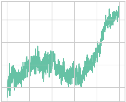
Head 9
