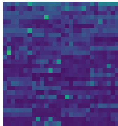
Longbench
