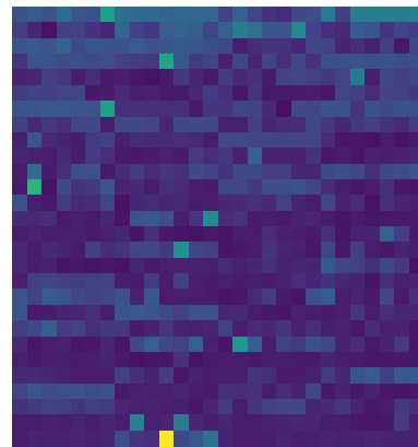
Pg19
