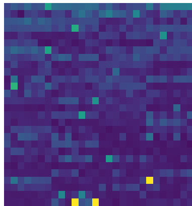
Booksum
