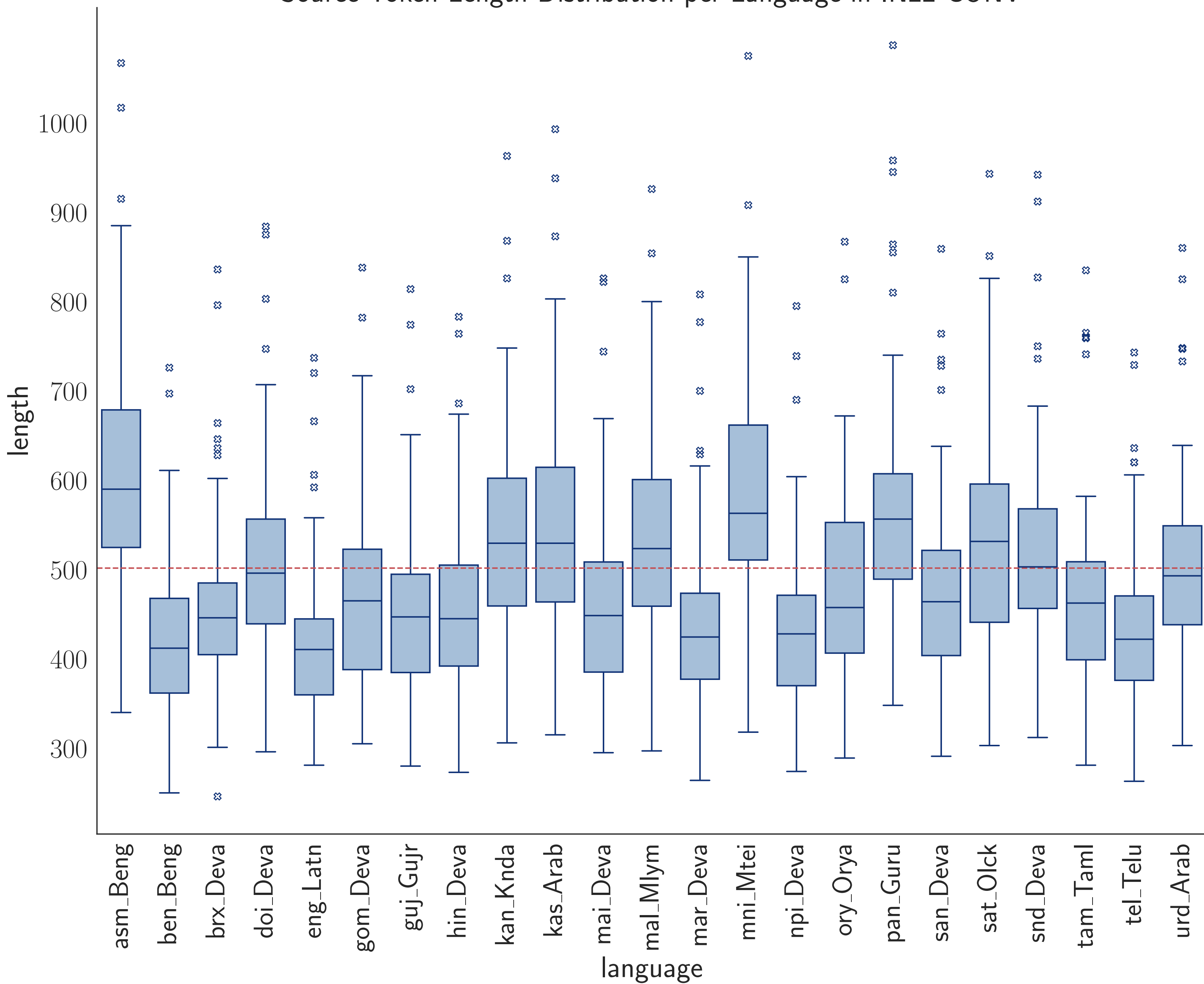
Source Token Length Distribution per Language in IN22 CONV
