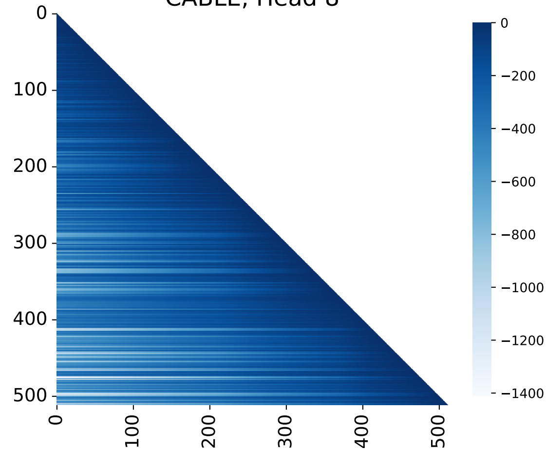
CABLE, Head 8
