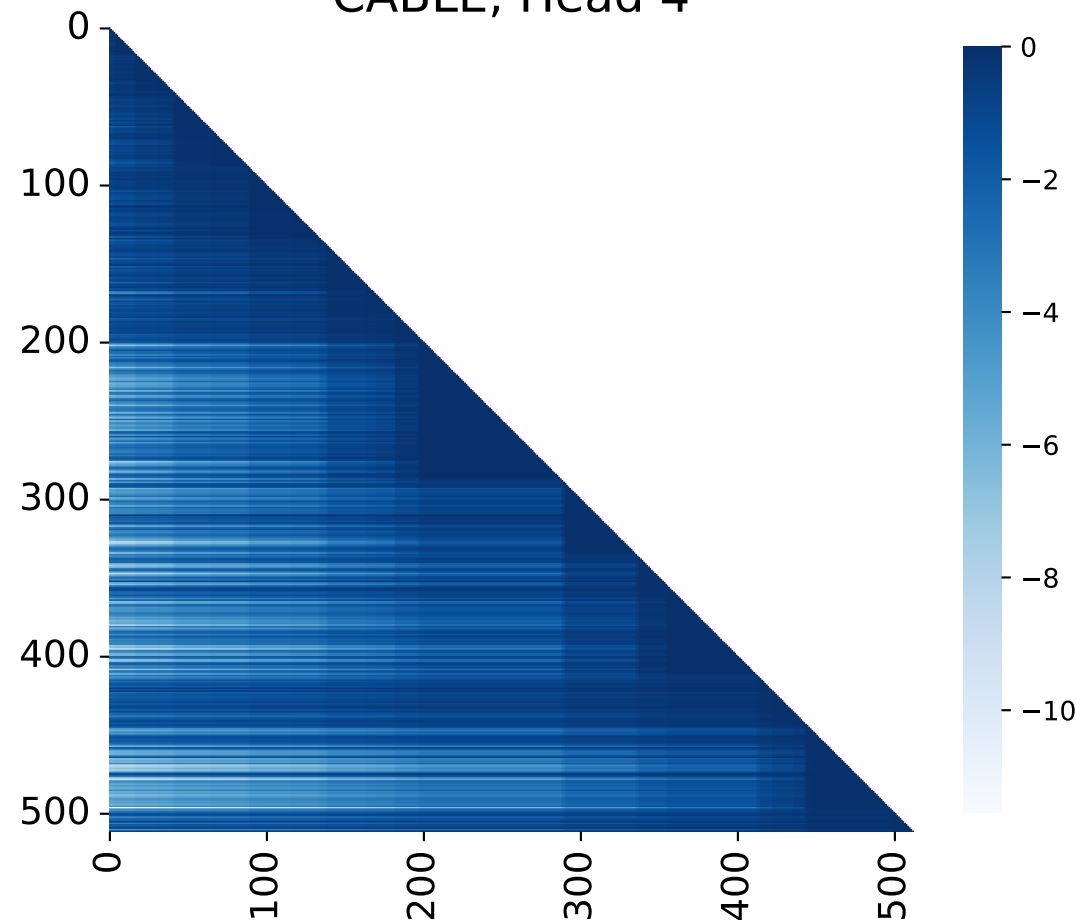
CABLE, Head 4
