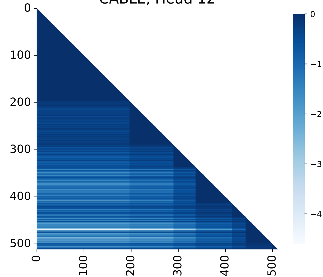
CABLE, Head 12
