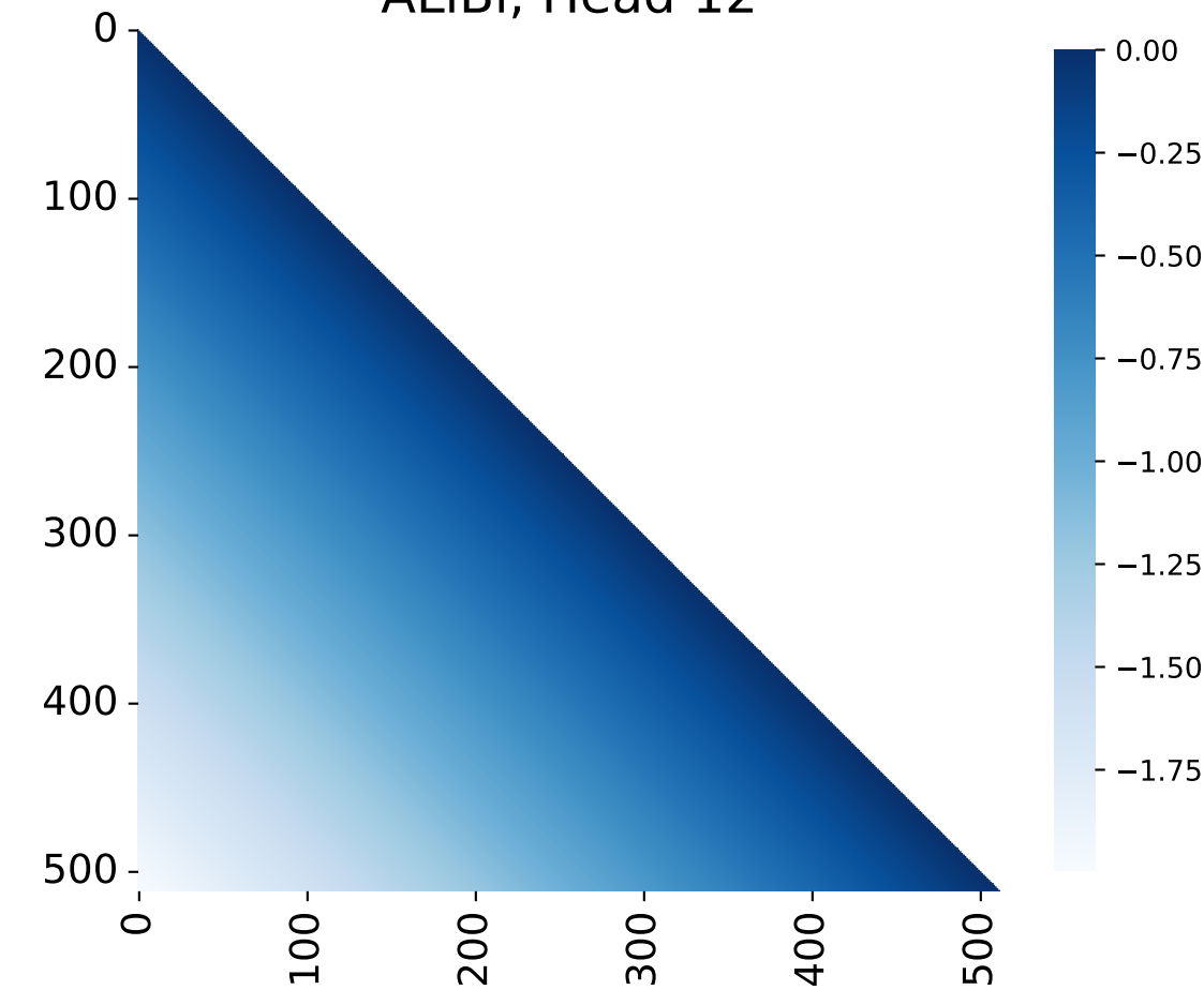
ALiBi, Head 12
