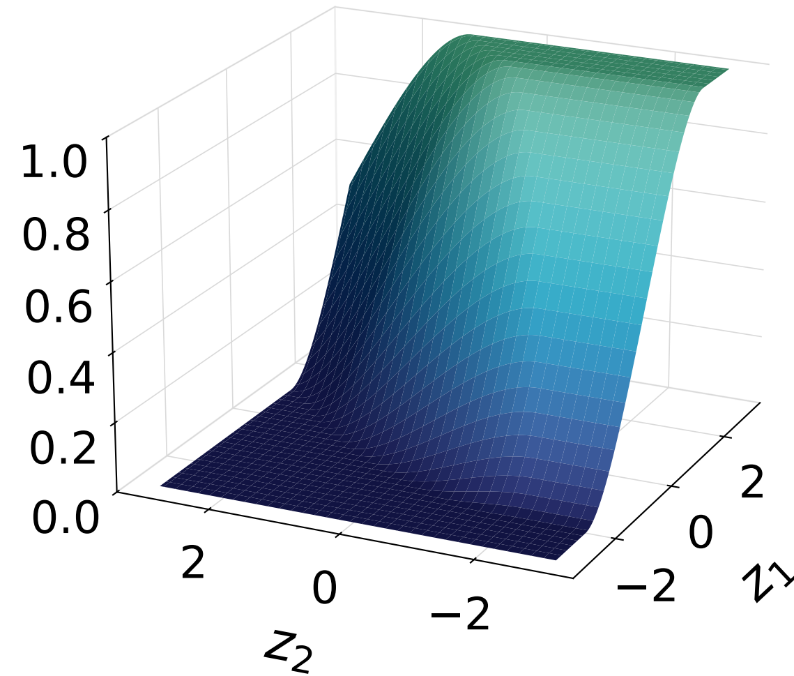
1.5-entmax
