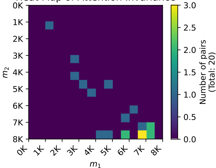
Heat Map of Attention Invariance
