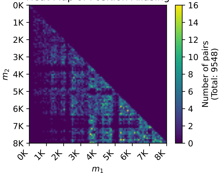
Heat Map of Position Aliasing
