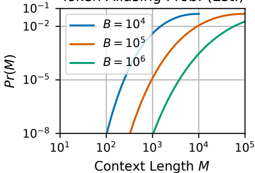
Token Aliasing Prob. (Est.)
