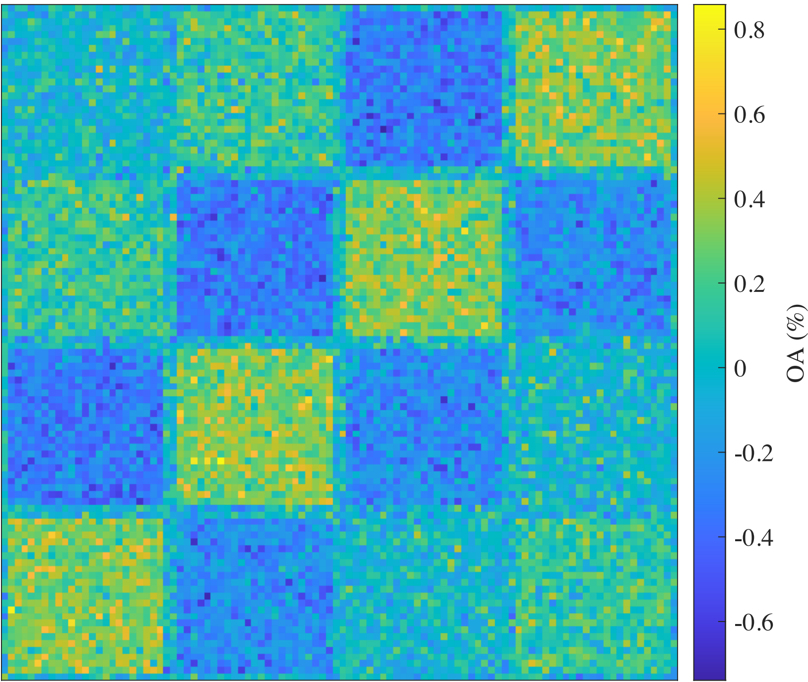
First Principal Component Scores
