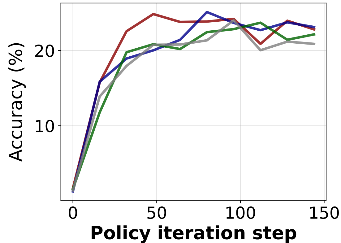
Average benchmark score
