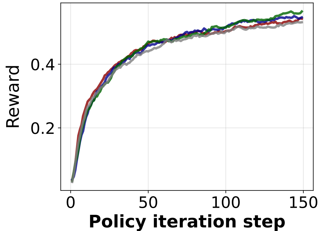
Training reward
