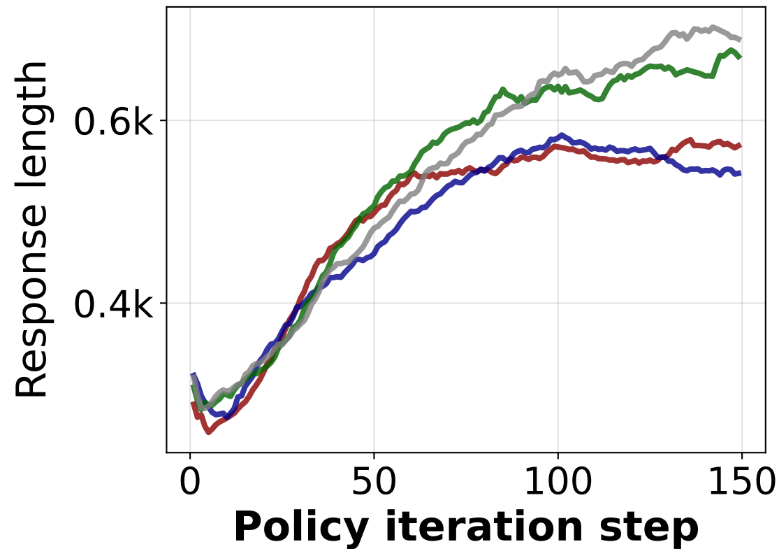
Training length
