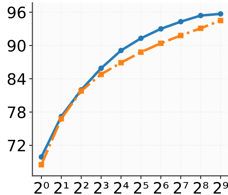
HumanEval++
