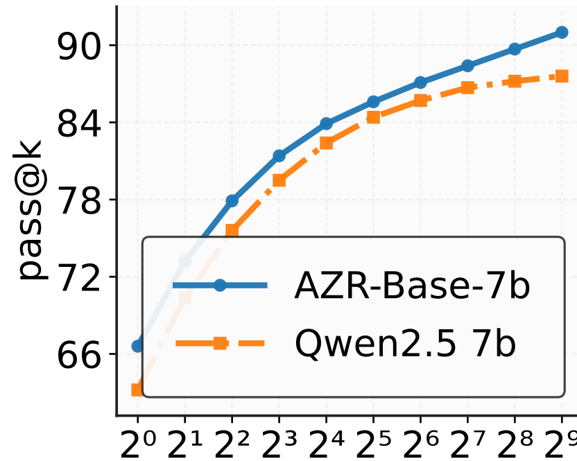
MBPP++
