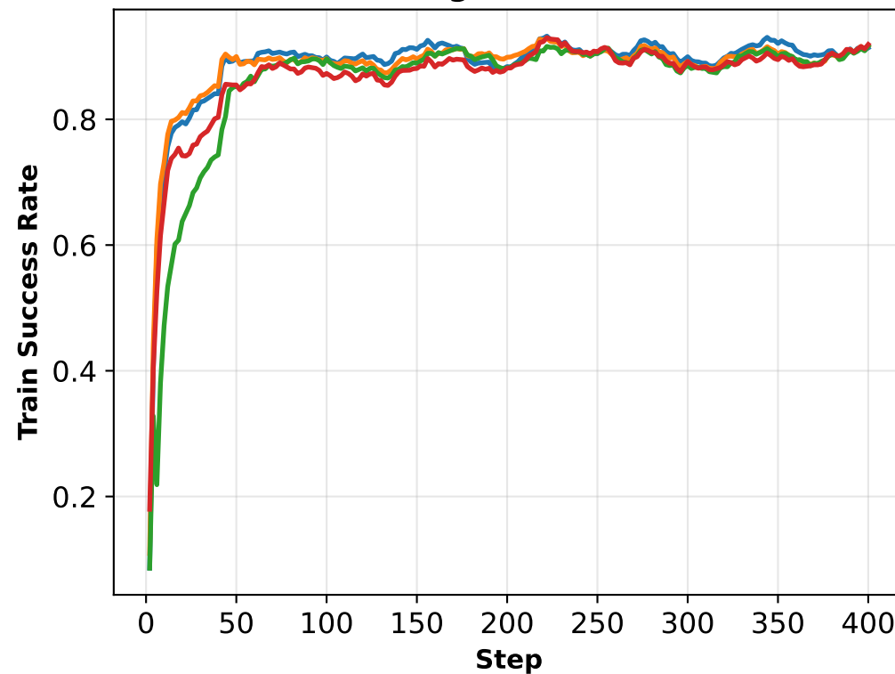
(a) Agentic Train
