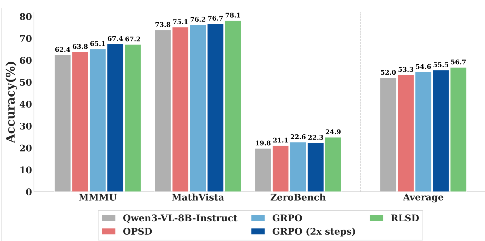
(b) Performance comparison on reasoning tasks.
