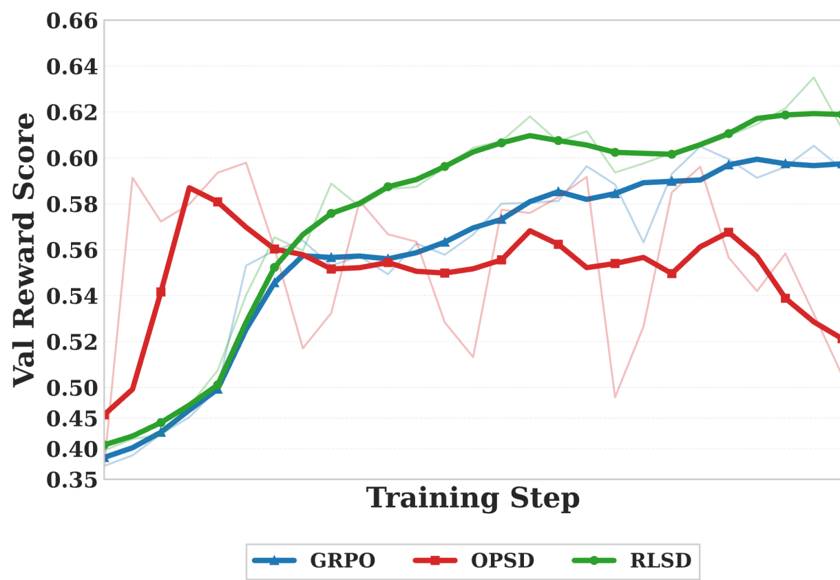
(a) Average performance dynamics on the validation set.
