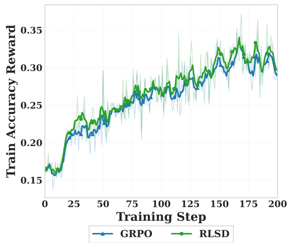
(a) Training reward dynamics comparison.
