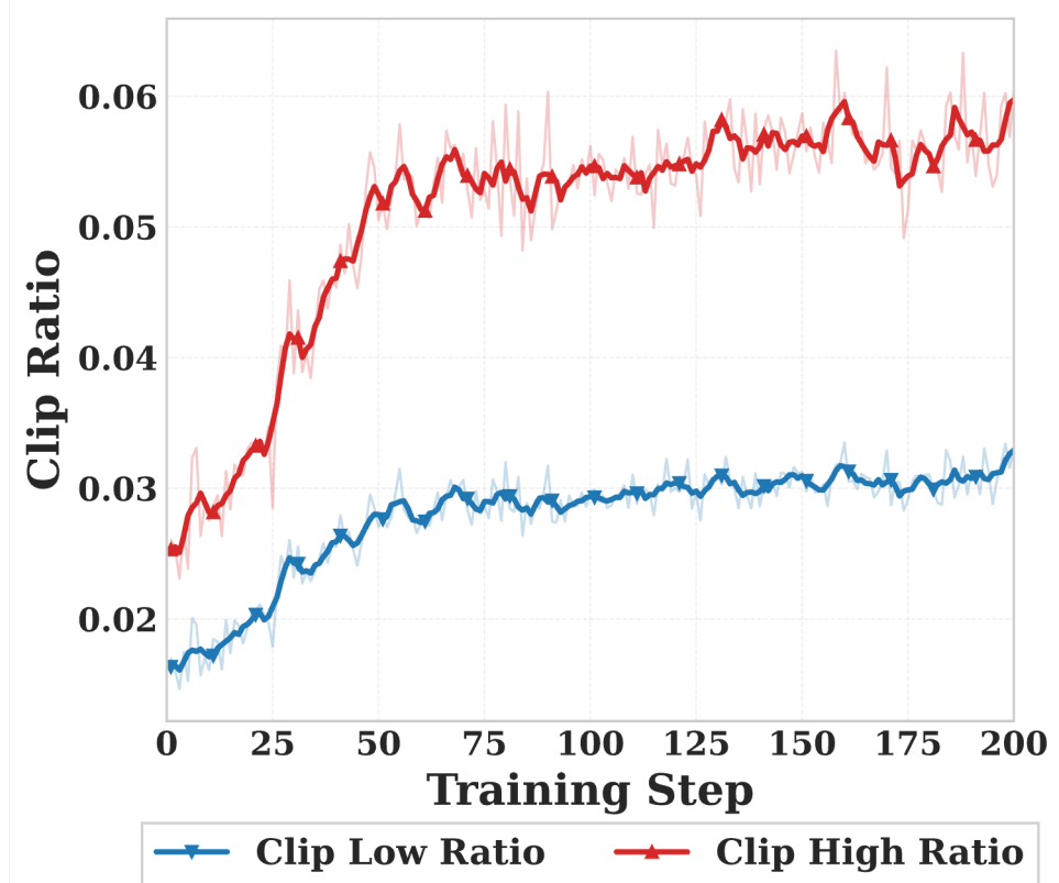
(c) Clip ratios on credit assignment
