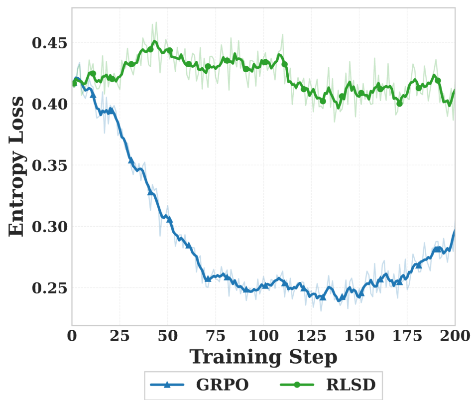
(b) Training entropy dynamics comparison.
