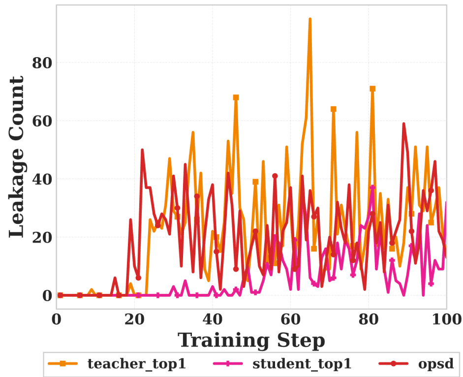
(a) Leakage occurrence dynamics.
