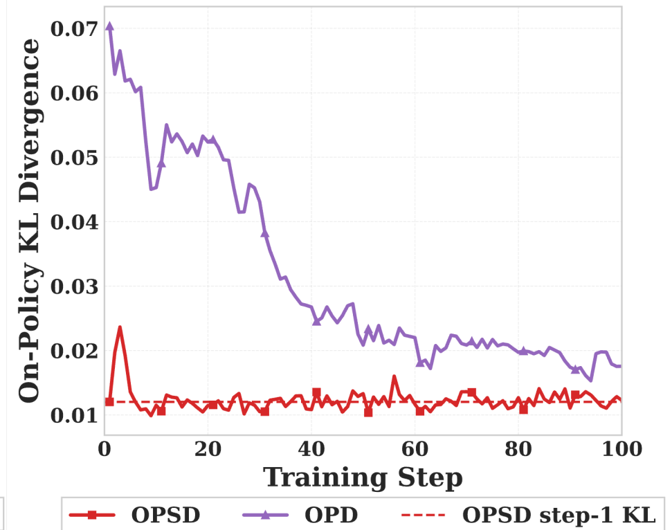
(c) KL Divergence comparison.
