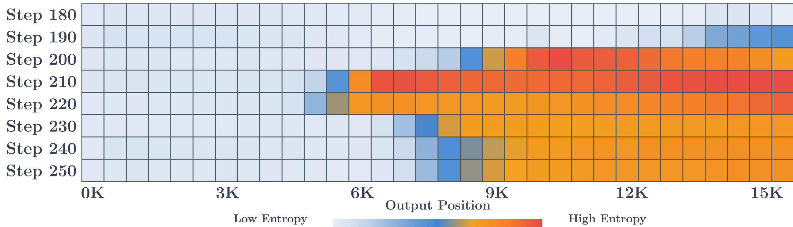
Student Entropy Heatmap
