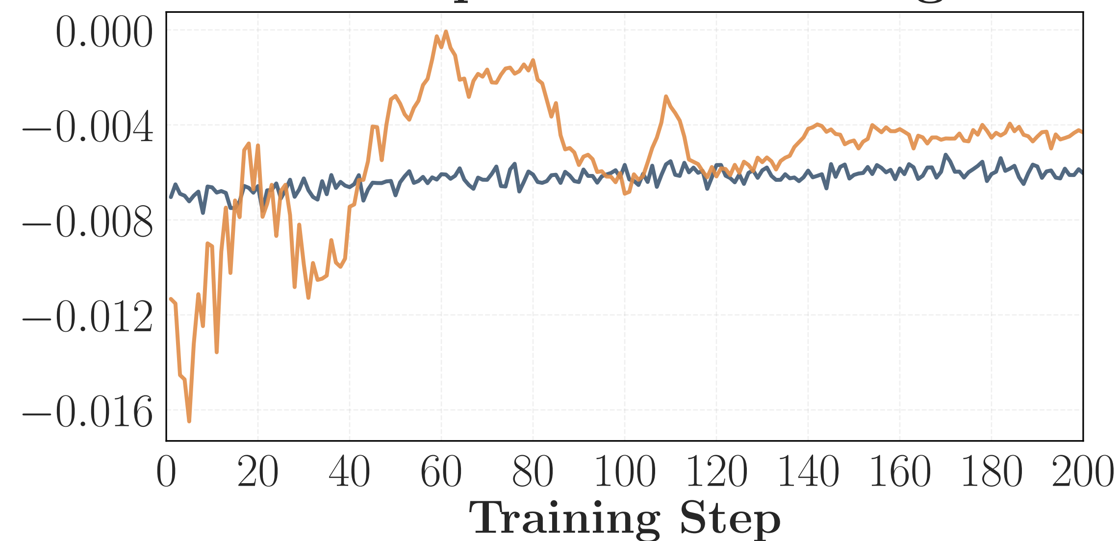
Overlap-Token Advantage
