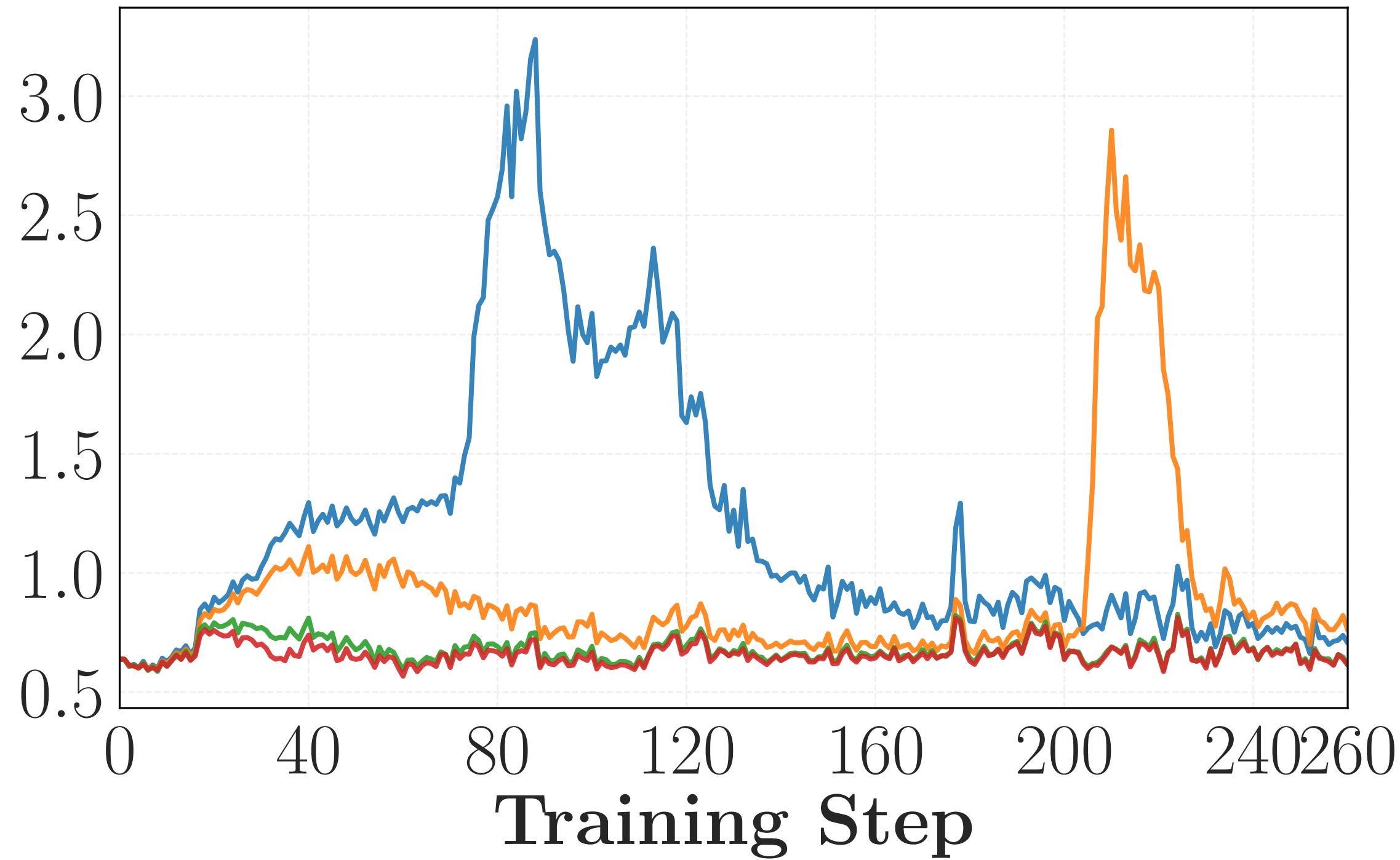
Student Entropy
