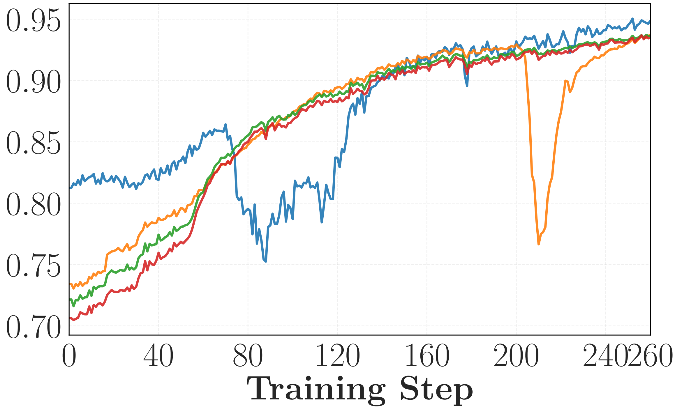
Overlap Ratio
