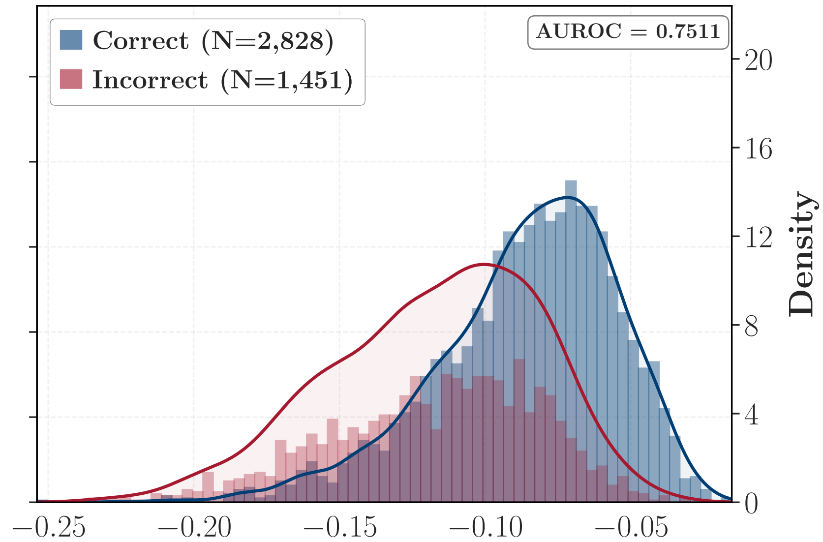
R1-Distill-7B as Teacher
