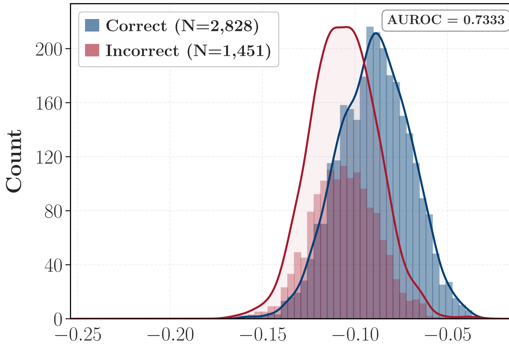
JustRL-1.5B as Teacher
