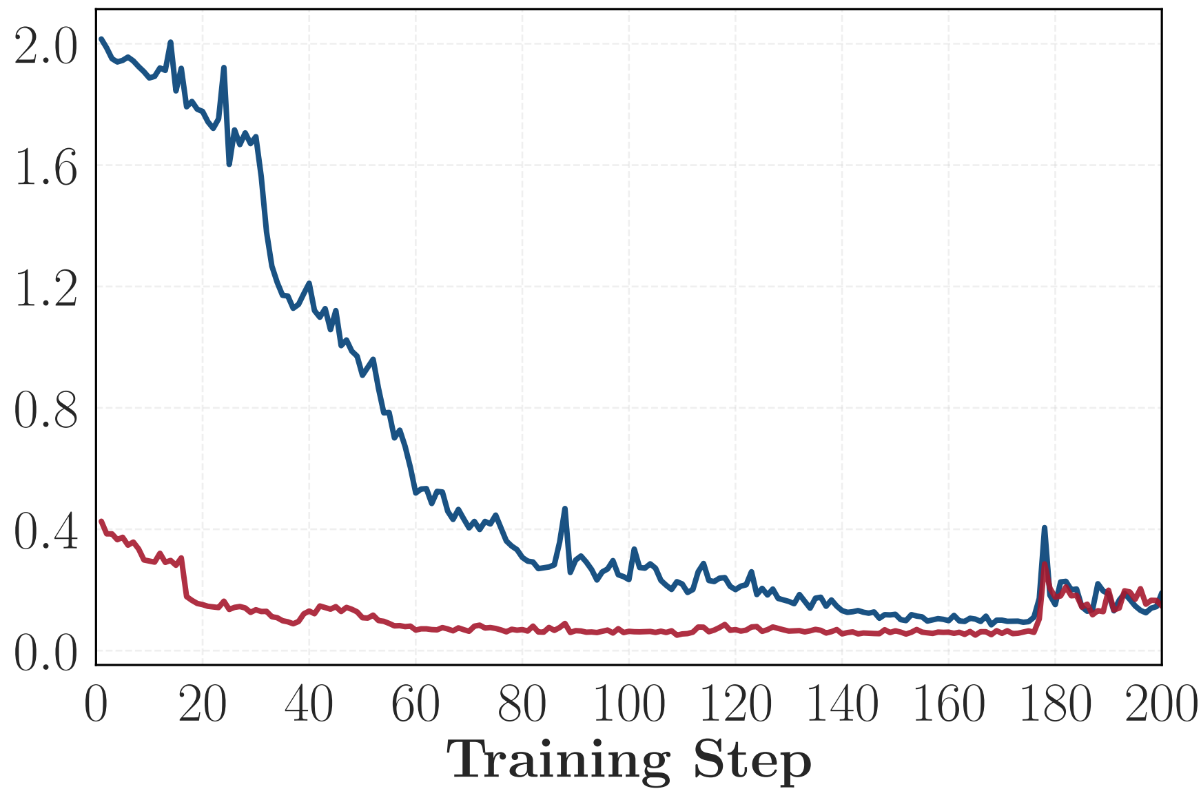
PG Loss
