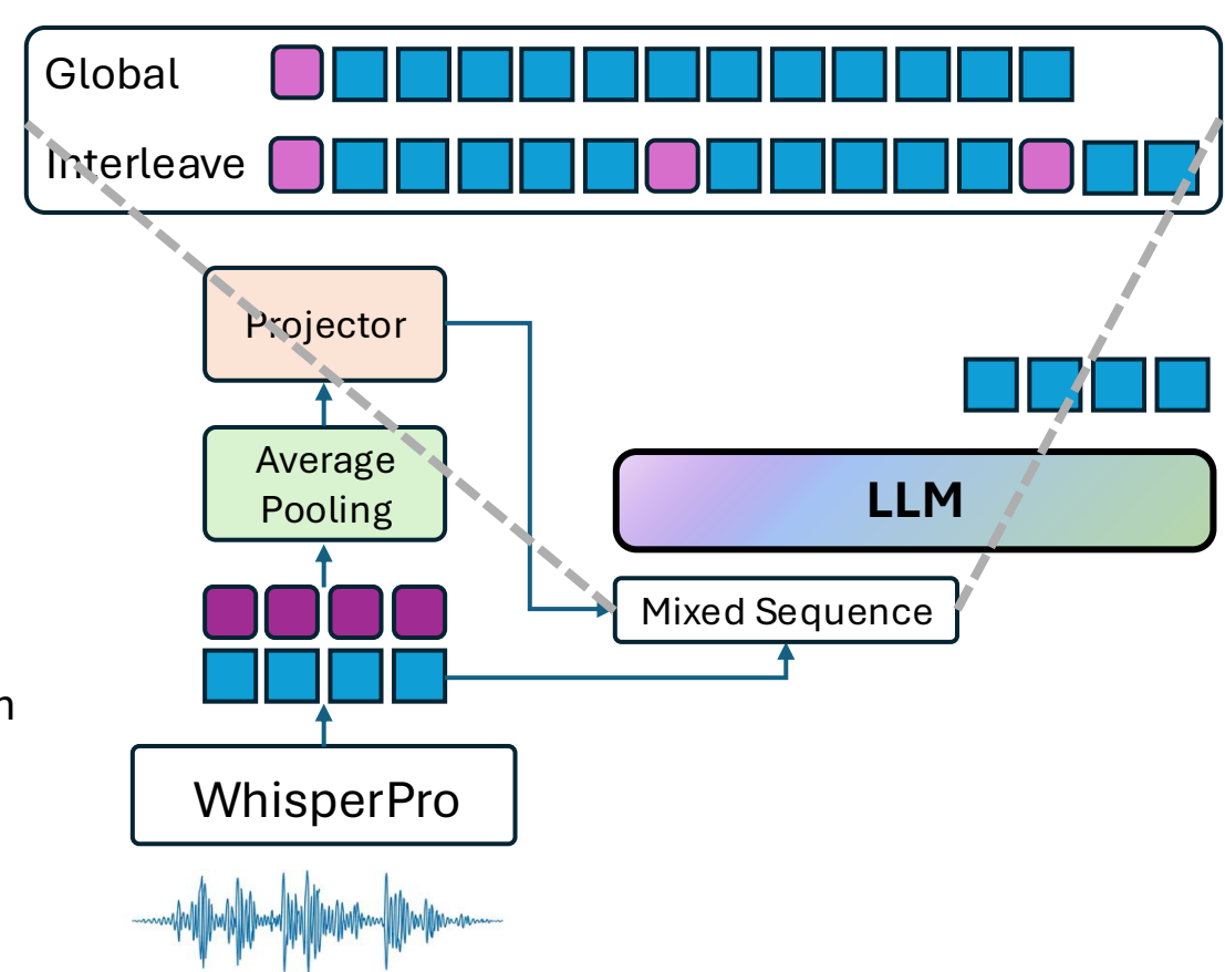
(b) TextPro-SLM Architecture
