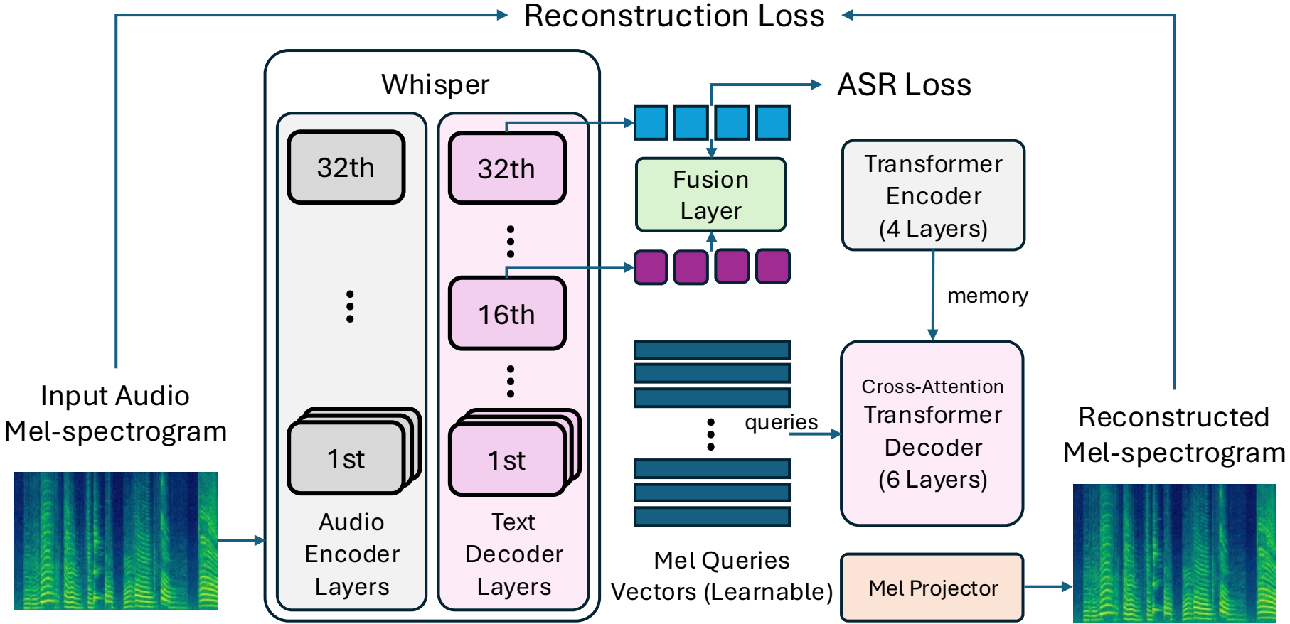
(a) WhisperPro Architecture
