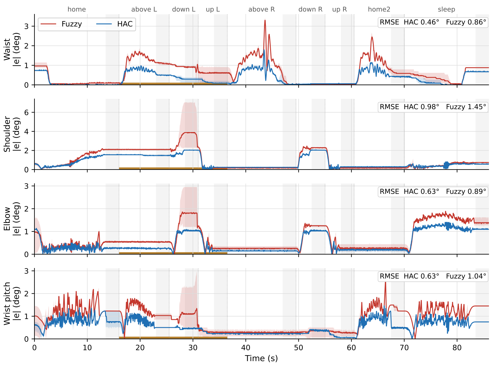
Absolute tracking error over the full slow pick-and-place cycle (mean of 3 trials, band = min-max; grey = hold phase)
