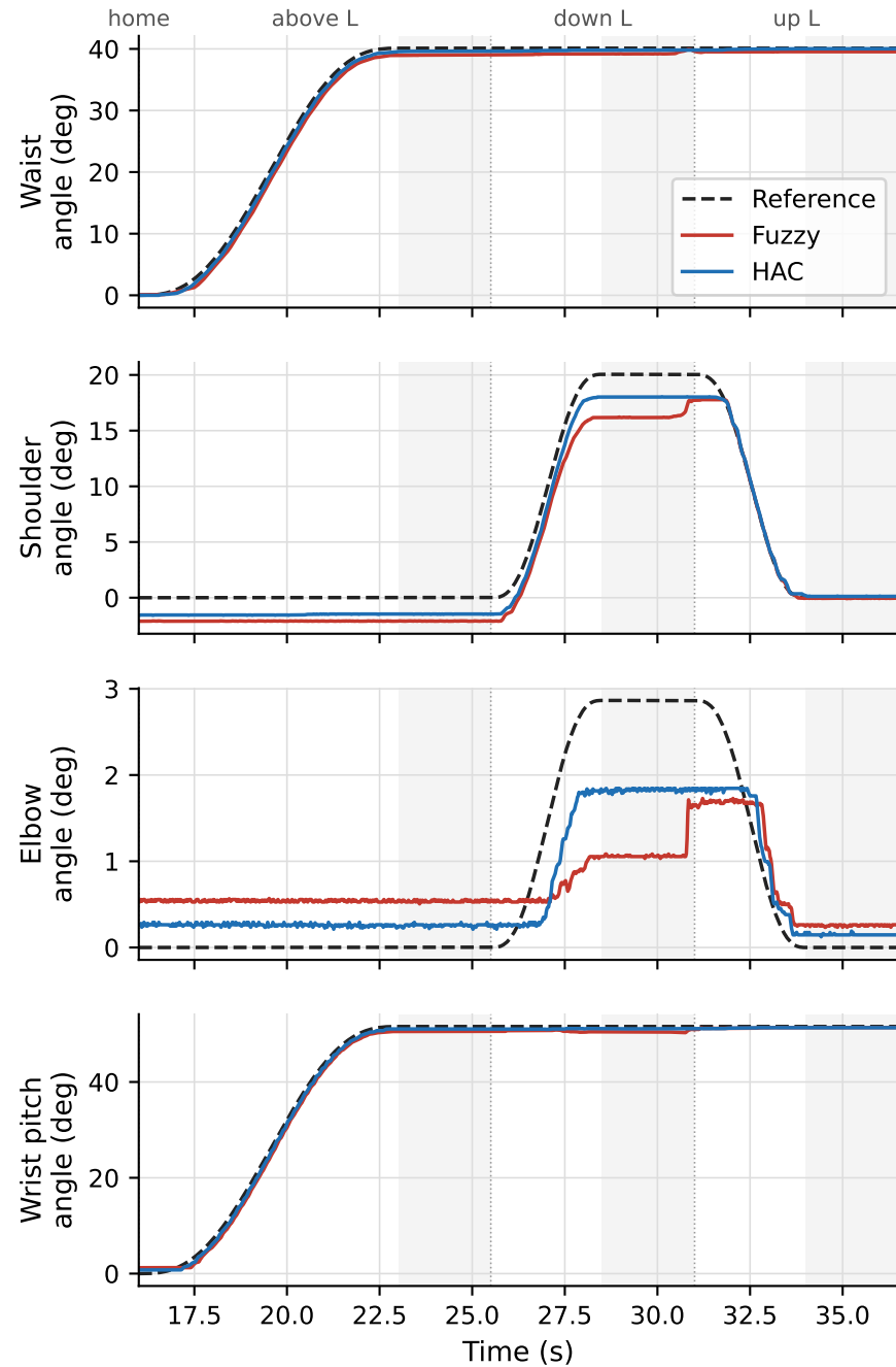
Joint position
